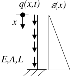
Figure 4.6 A bar and the corresponding compression shape, assuming linear elastic material response and a uniformly distributed load.
