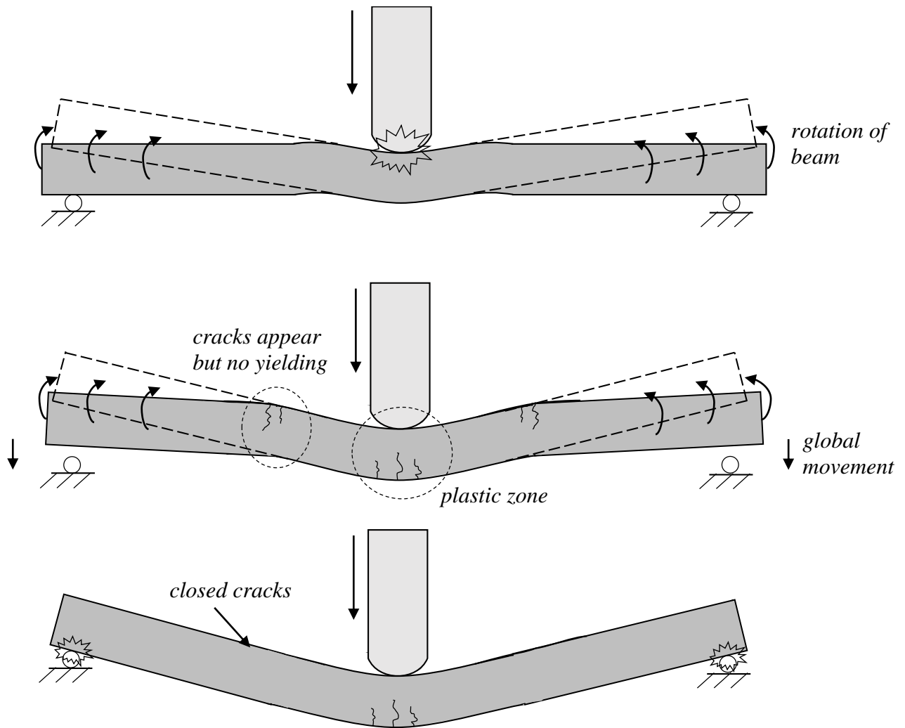
Figure 6.33 Elastic and plastic deformation of the bar shortly after impact, during the reaction wave propagation.
