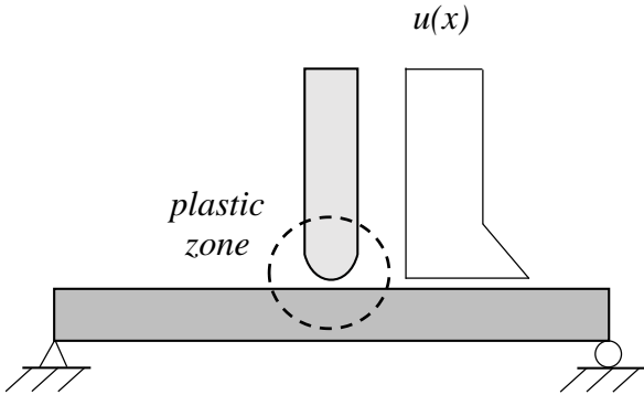
Figure 4.14 Displacement shape of the bar in the experiment.
