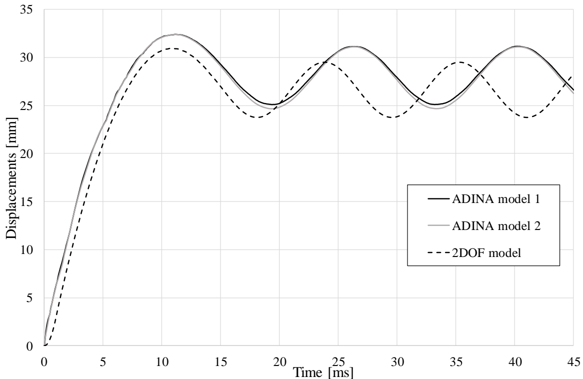
Figure 6.10 Maximum displacements of the ADINA models and 2DOF model, respectively.
