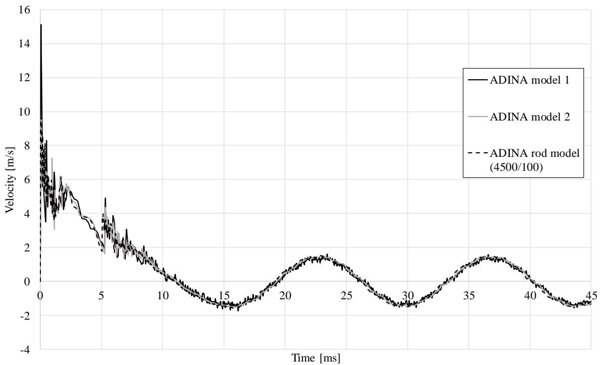
Figure D.6 Midpoint velocity over time for ADINA models.
