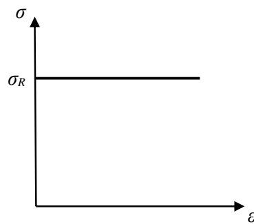
Figure 2.3 Stress-strain relation for an ideal plastic material.
