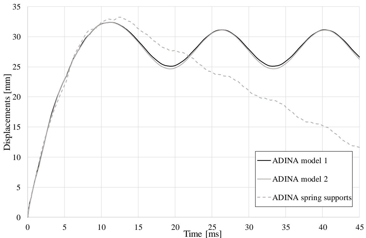
Figure 7.17 Displacement of midpoint over time for the ADINA models.
