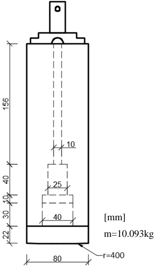
Figure 5.4 Cross section of the drop weight.
