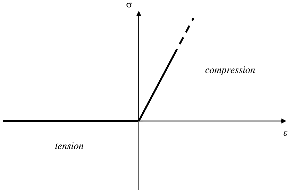
Figure 5.13 Behaviour of spring in the FE-models.
