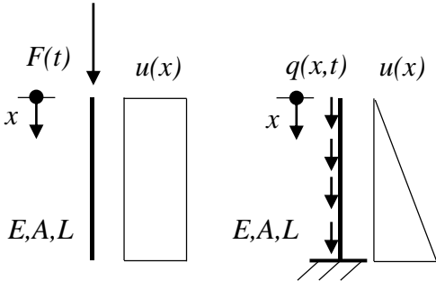
Figure 4.13 Different displacement shapes of a bar, depending on the applied load.
