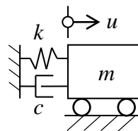
Figure 3.12 Damped spring-mass system.
