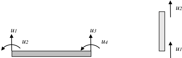
Figure 4.5 Degrees of freedom for a beam and a bar, respectively.
