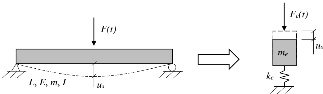
Figure 4.2 A beam transformed into an equivalent SDOF system.
