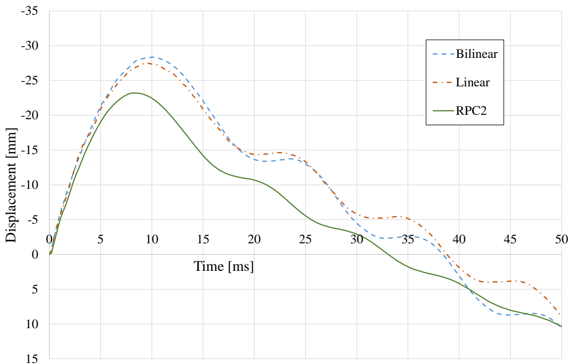
Figure 7.3 Displacement as a function of time for bilinear and linear damage curves compared to test results of RPC2.
