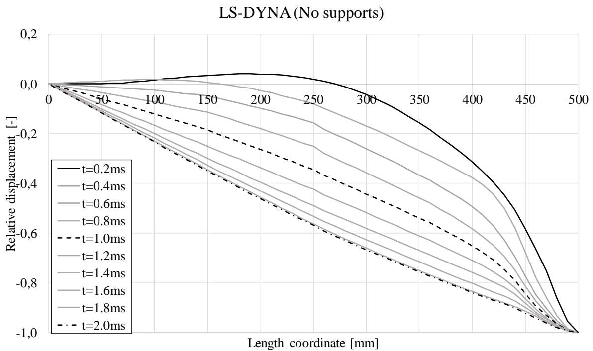
Figure D.15 Displacement over length for LS-DYNA model with no supports,
