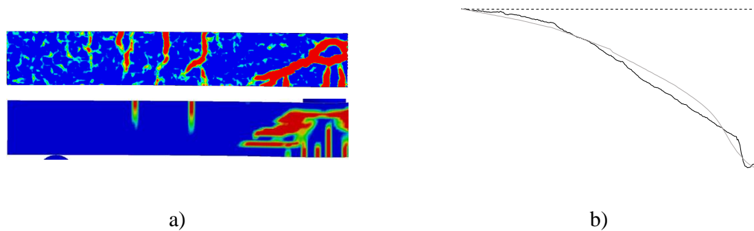
Figure D.30 Response after 0.8 ms: a) Crack pattern for RPC2 and LS-DYNA, respectively and b) Displacement shape for RPC2 (black) and LS-DYNA (grey).
