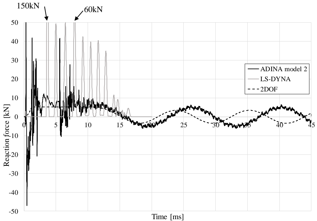
Figure 6.16 Reaction force over support for the numerical models.
