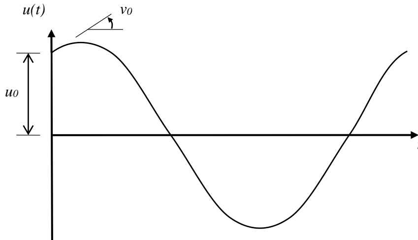
Figure 3.11 Free vibration of an undamped SDOF system.
