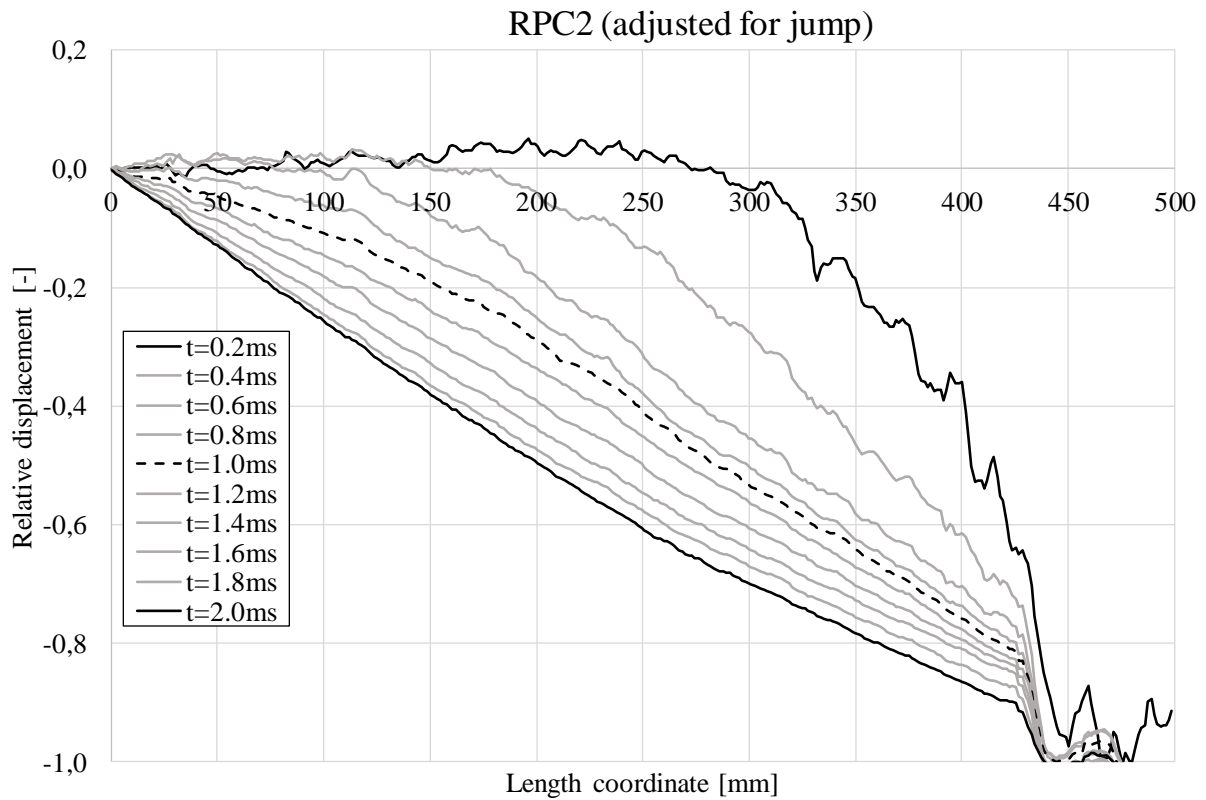
Figure D.22 Displacement over length of RPC2.
