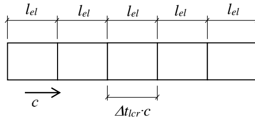
Figure 3.23 Maximum critical time step.
