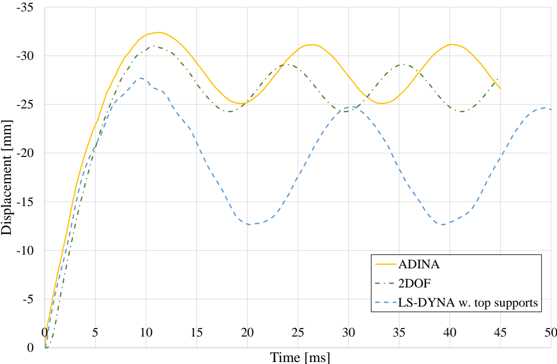
Figure 7.8 Displacement as a function of time from ADINA, 2DOF calculations and LS-DYNA model with top supports.
