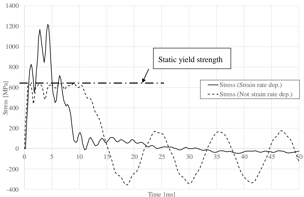
Figure 7.14 Stress in reinforcement.
