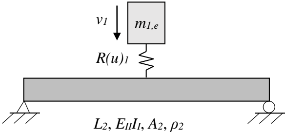
Figure 5.6 The model used in the first ADINA analysis (ADINA model 1), with a point mass hitting a beam.
