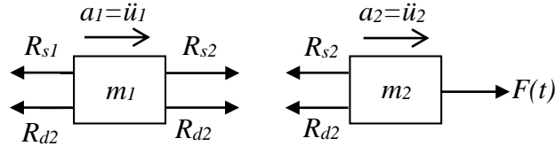
Figure 3.22 Free body diagram of the system.
