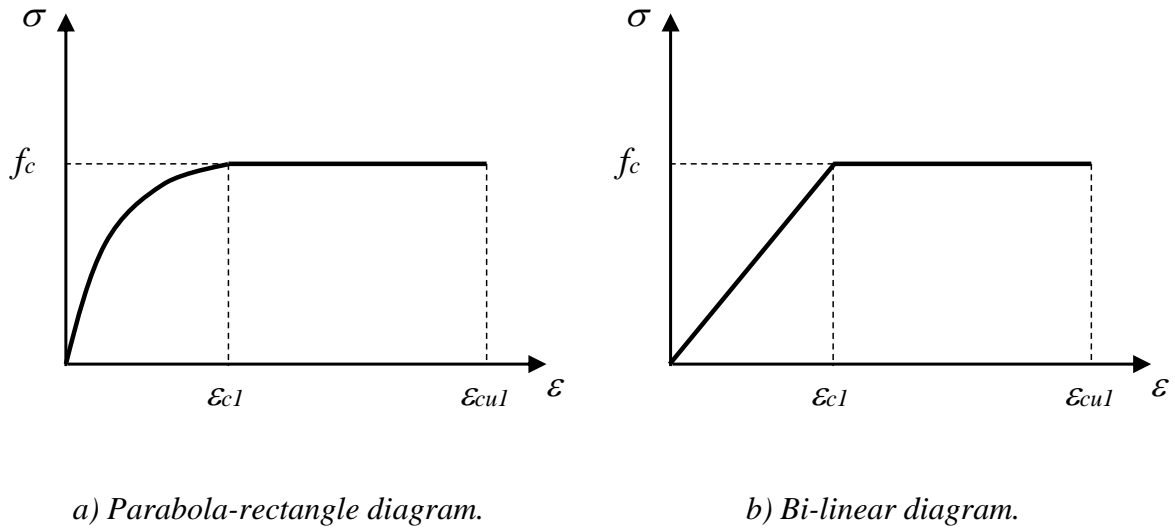
Figure 2.9 Simplified stress-strain relations of concrete.
