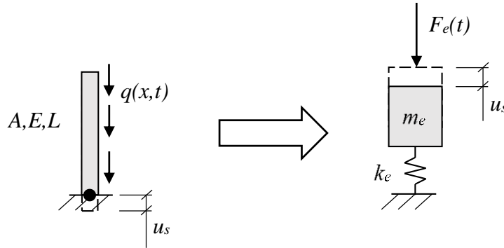
Figure 4.8 A bar transformed into an equivalent SDOF system.
