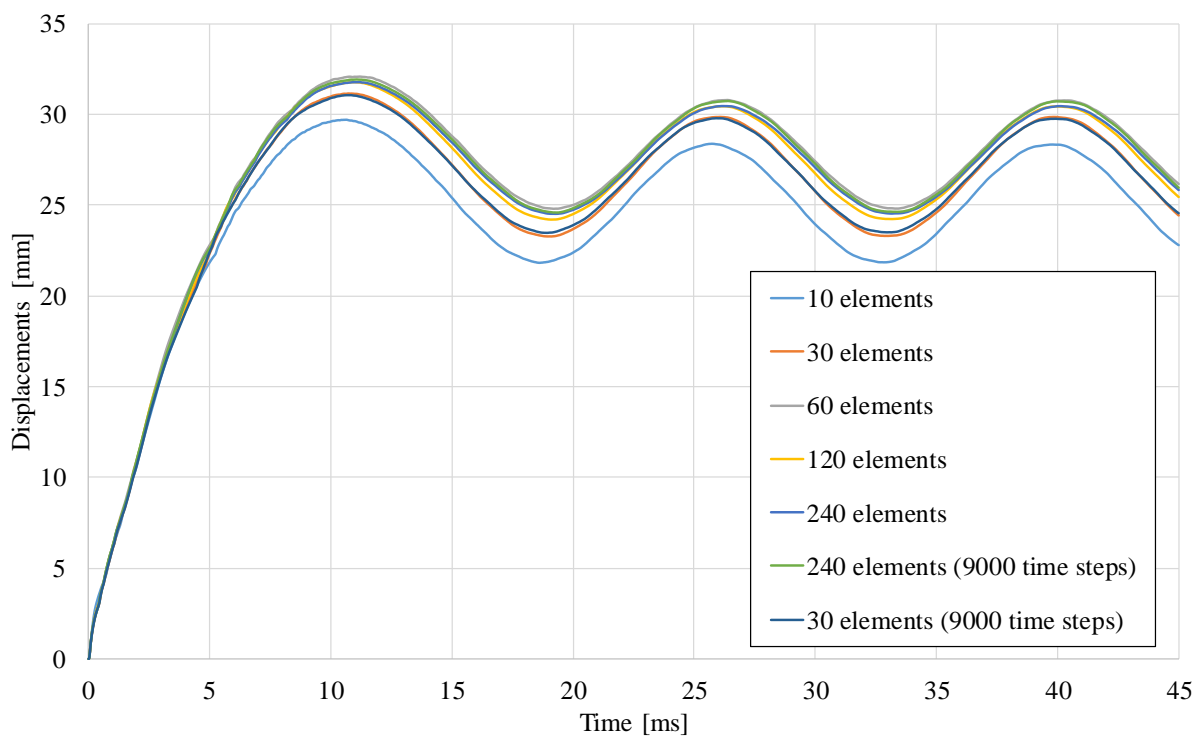
Figure H.4 Convergence study of number of elements for the beam in ADINA.
