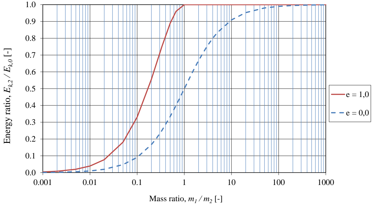
Figure 3.20 Energy ratio as a function of mass ratio for a purely elastic case ( e = 1 ) and a purely plastic case ( e = 0 ).
