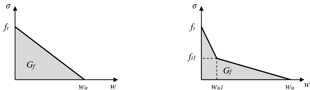
a) Linear fracture energy damage model b) Bilinear fracture energy damage model
