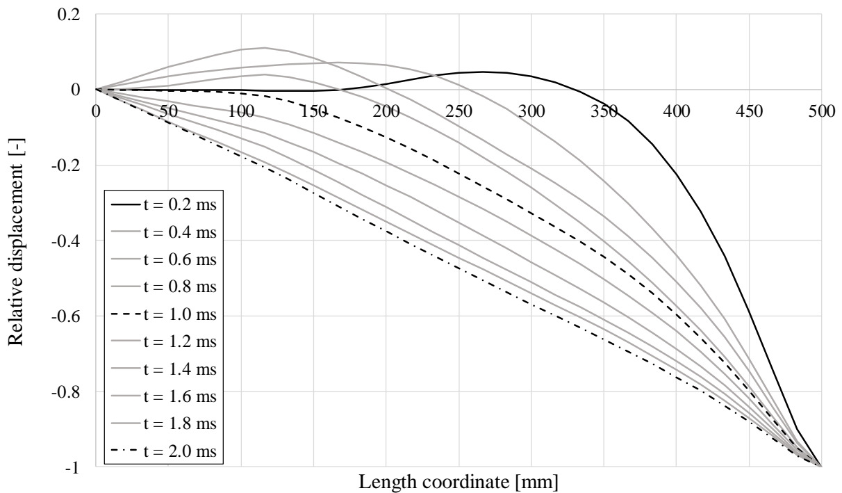
Figure 6.27 Displacement shape of the beam in ADINA model 1 during the first 2 ms.
