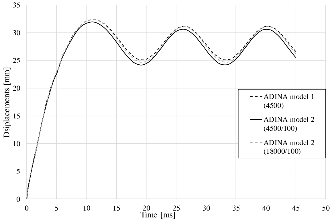
Figure 5.15 Convergence study for ADINA model 2, different time steps.
