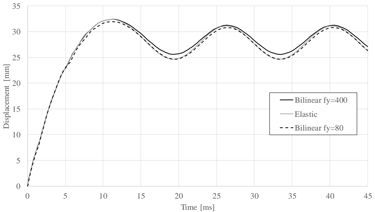
Figure H.3 Response of the midpoint using different material models for the rod in ADINA model 2.
