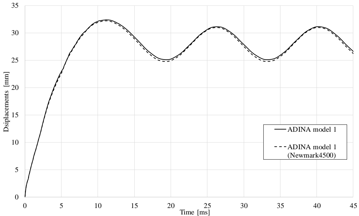
Figure H.1 Comparison of the response in ADINA when using Bathe or Newmark method as direct integration-solver.
