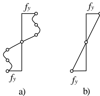
Figure 5.8 Stress distribution using a) 7 integration points b) 3 integration points. Based on (Carlsson & Kristensson 2012).
