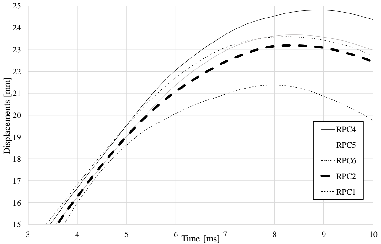
Figure 6.7 Maximum displacement for the beams in the experiment, with RPC2 highlighted.
