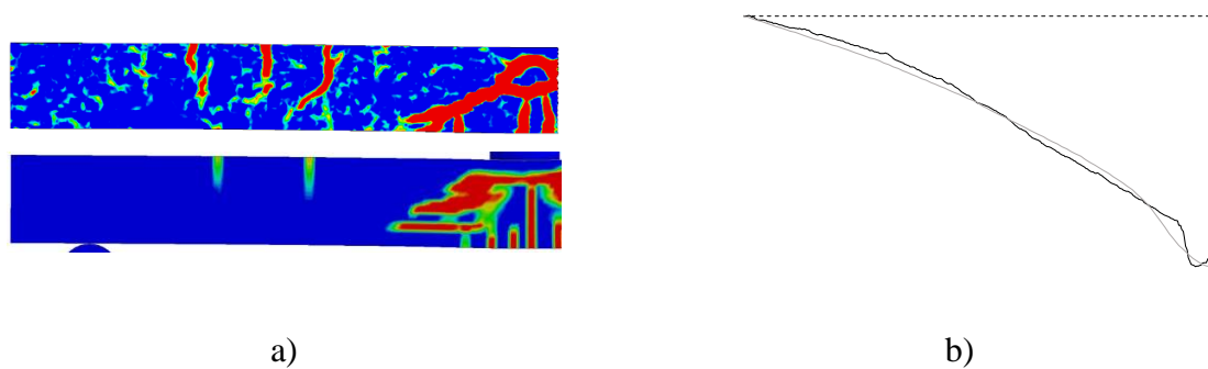
Figure D.31 Response after 1.0 ms: a) Crack pattern for RPC2 and LS-DYNA, respectively and b) Displacement shape for RPC2 (black) and LS-DYNA (grey).
