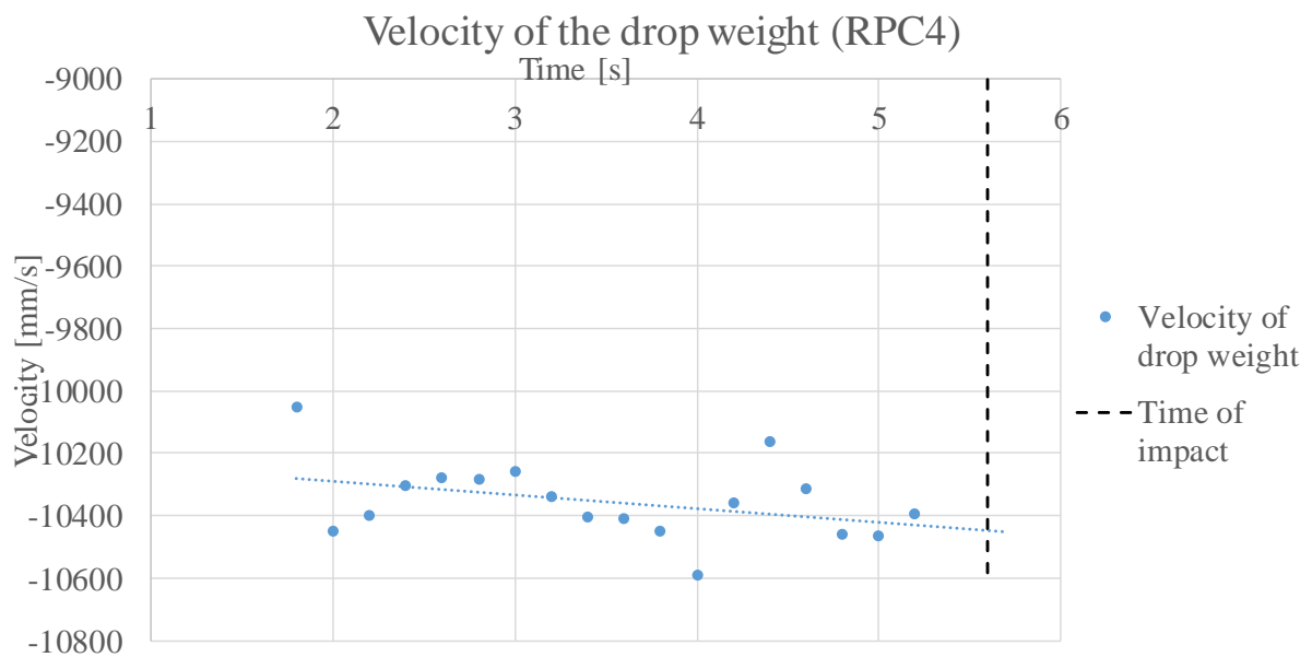
Figure D.26 Derivation of a value for the velocity at impact in the experiment.
