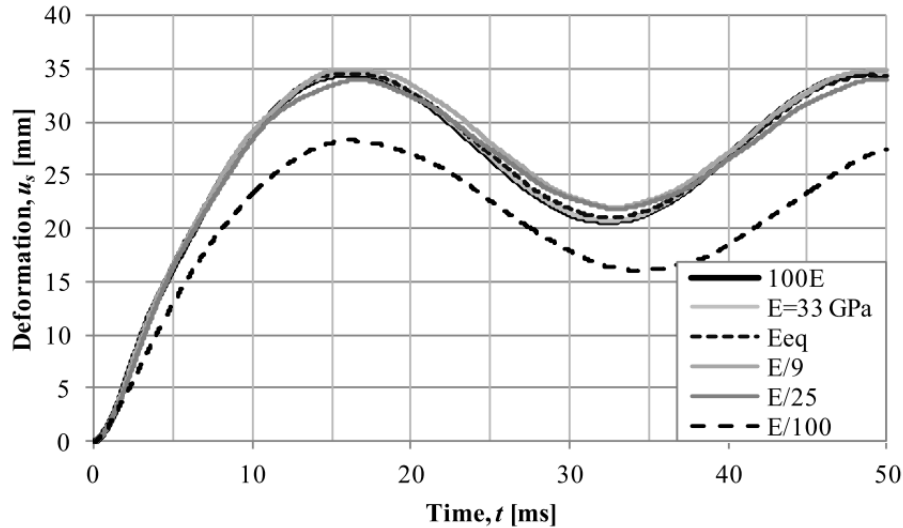
Figure 5.12 Study of the influence of different E for the response of a beam subjected to a point load (Andersson & Karlsson 2012).
