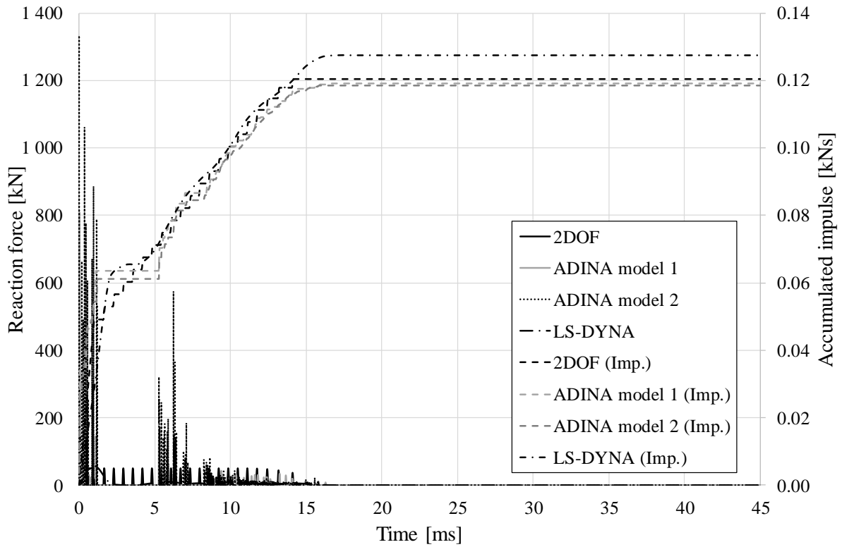
Figure 6.2 Reaction force/Accumulated impulse (denoted as imp.) for the analytical models.
