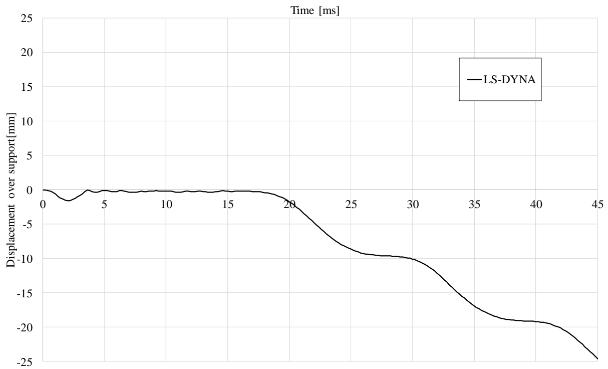
Figure D.13 Support displacement over time of LS-DYNA models
