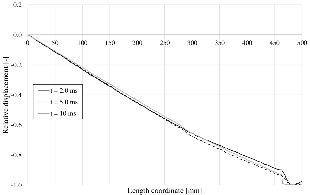
Figure 6.34 Displacement shape at different times for RPC2.
