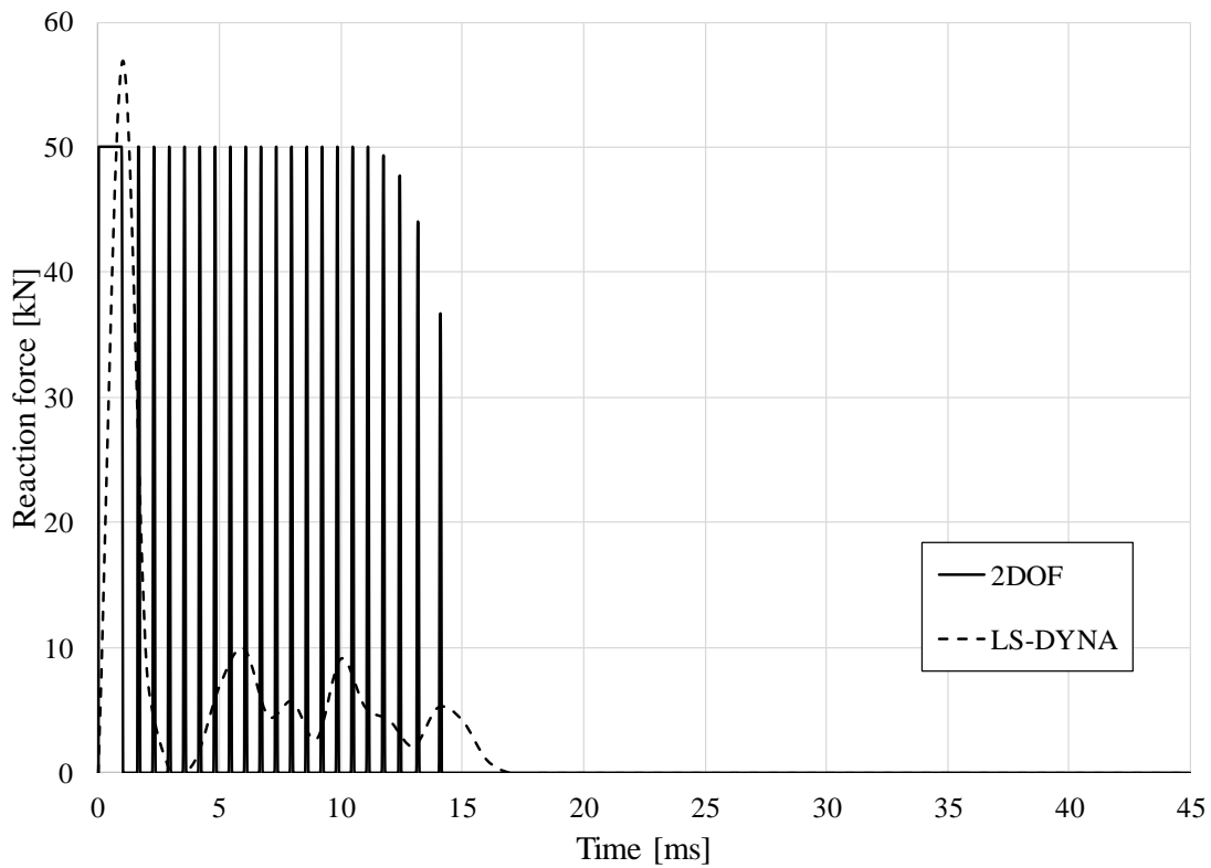
Figure 6.3 Reaction force of 2DOF and LS-DYNA model only.
