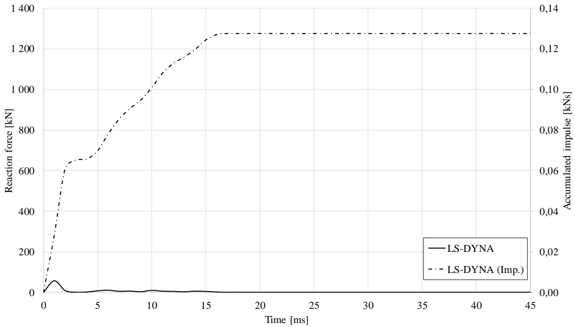
Figure D.19 Reaction force/Accumulated impulse for LS-DYNA model.
