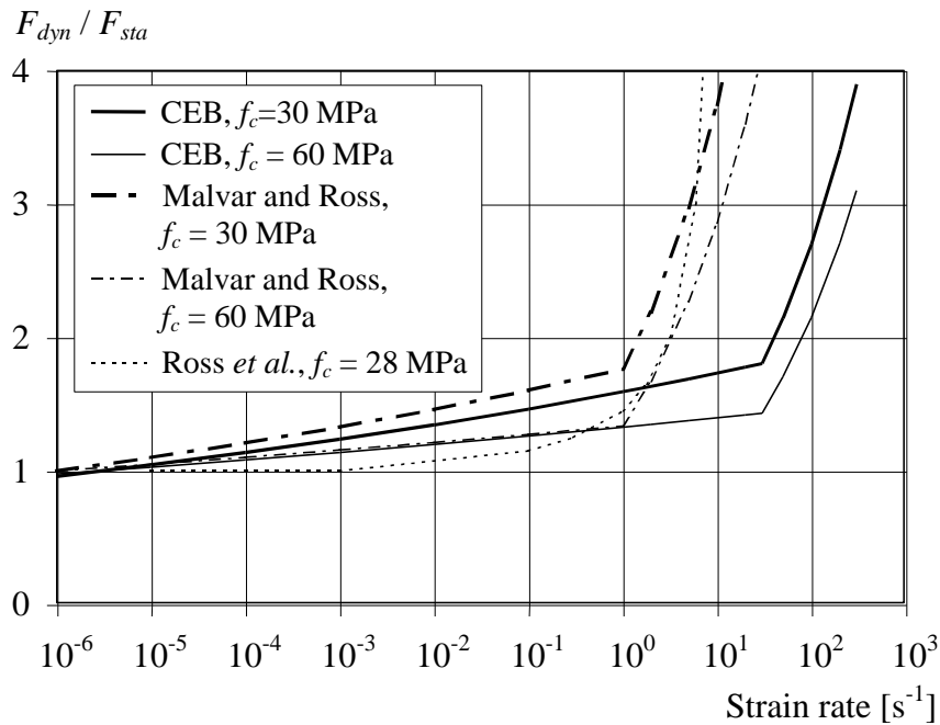
Figure 3.27 Different studies of the dynamic implication factor-strain rate relations for concrete in tension. (Johansson 2000)
