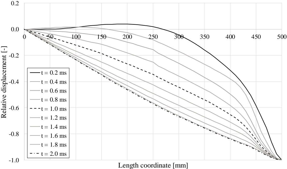
Figure 6.32 Displacement shape of the beam in the LS-DYNA model with no supports during the first 2 ms.
