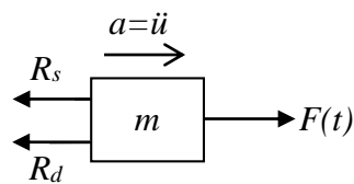
Figure 3.9 Free body diagram of the system.
