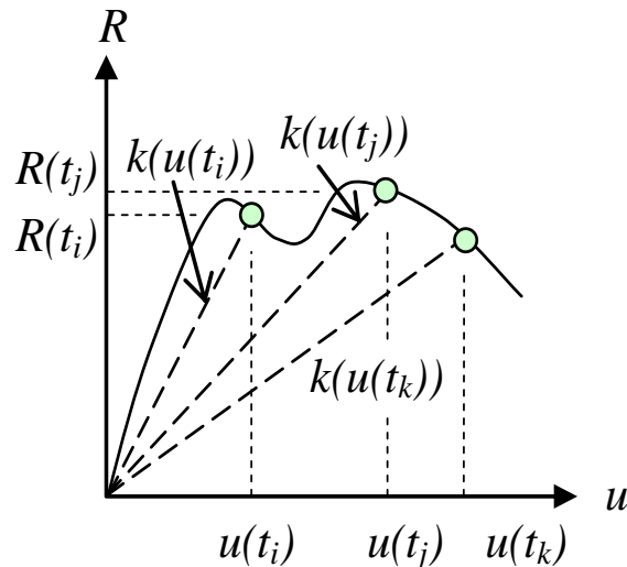
Figure 3.25 Secant stiffness k at time t for a system with an arbitrary response (Johansson & Laine 2012).
