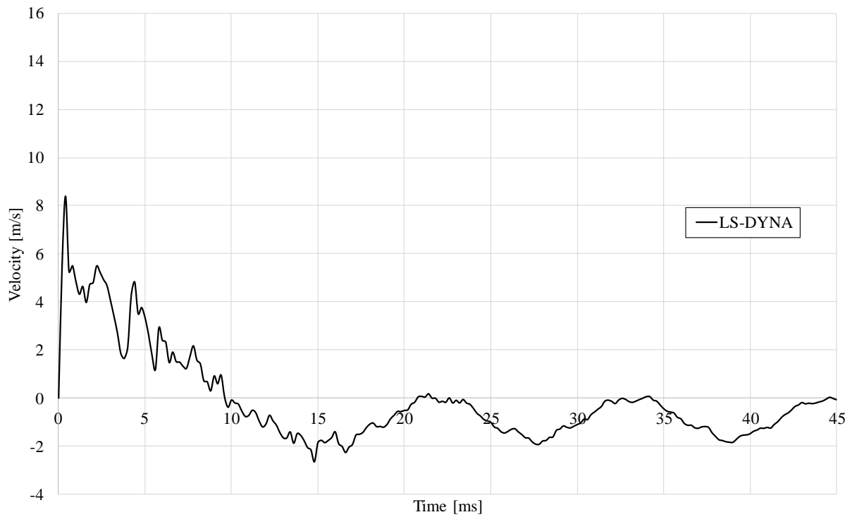
Figure D.16 Midpoint velocity in LS-DYNA model.
