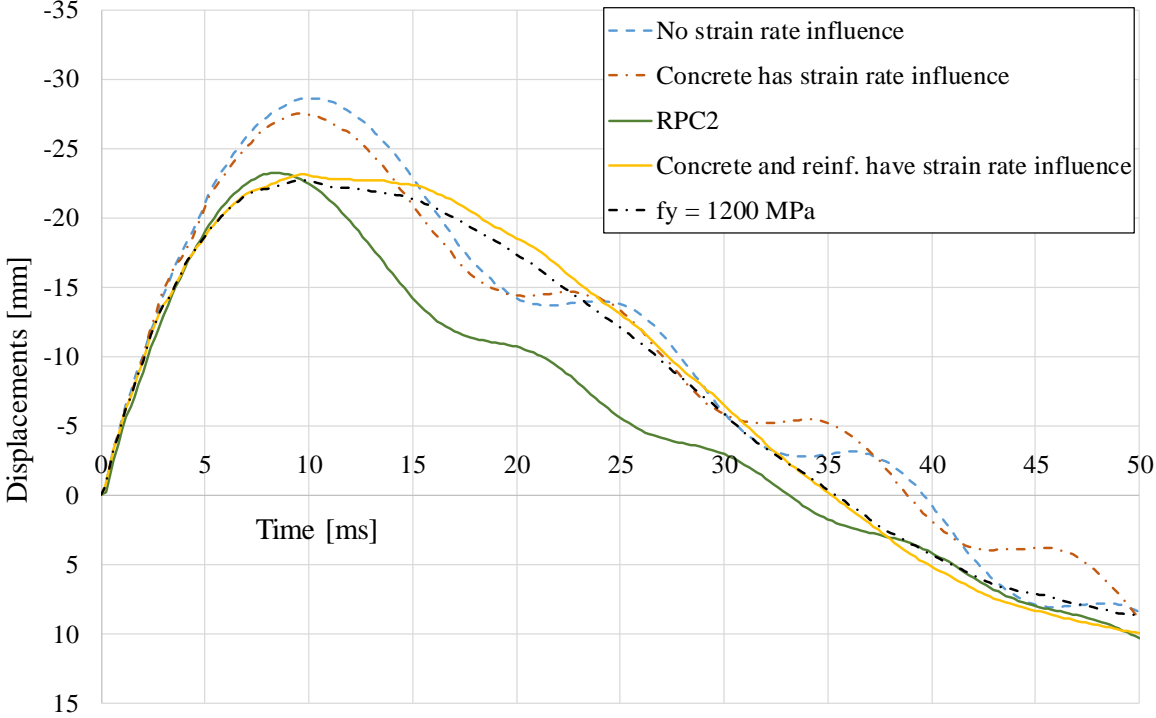
Figure 7.15 Displacement of midpoint as a function of time including response of the beam with reinforcement with increased yield strength.
