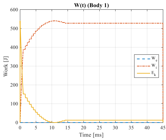
Figure D.2 Results from 2DOF model, continued.
