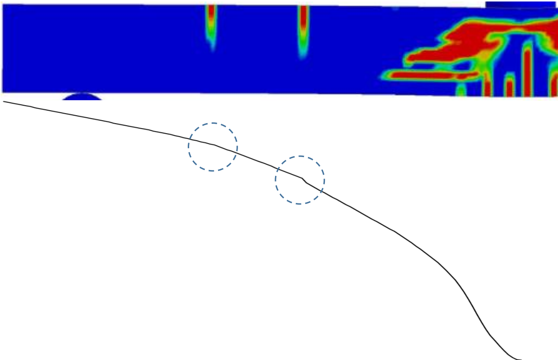
Figure 6.41 Crack pattern/displacement shape for LS-DYNA model after 0.8 ms, with the distinct curvature shifts, at the places where two top cracks appeared.
