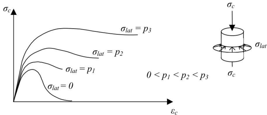
Figure 2.10 The influence of lateral confinement on concrete in compression, from (Ekengren et al. 2005).
