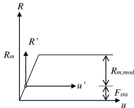
Figure 4.11 Influence of static loads on the dynamic response. Based on (Johansson 2014).
