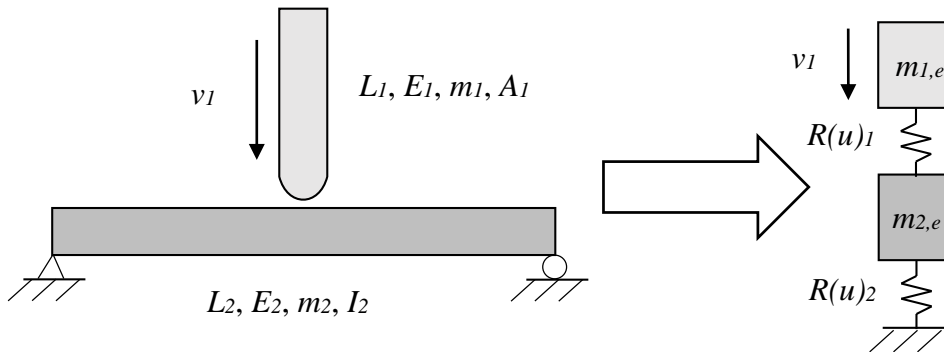
Figure 4.1 The beam-drop weight system and the equivalent transformed mass-spring system.
