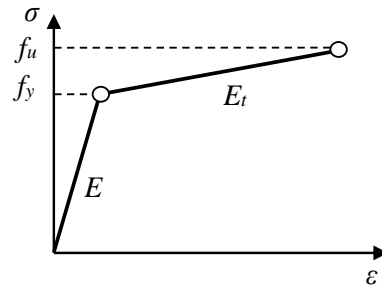
Figure 5.21 The bilinear elastoplastic behaviour of material model 003 – PLASTIC _ KINEMATIC.
