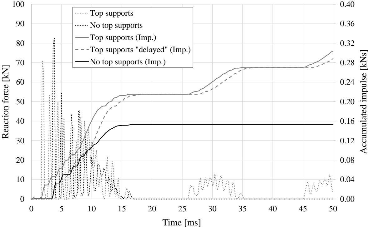
Figure 7.9 Reaction force and accumulated impulse in the beam - bottom support interface for both the model with top supports and without.
