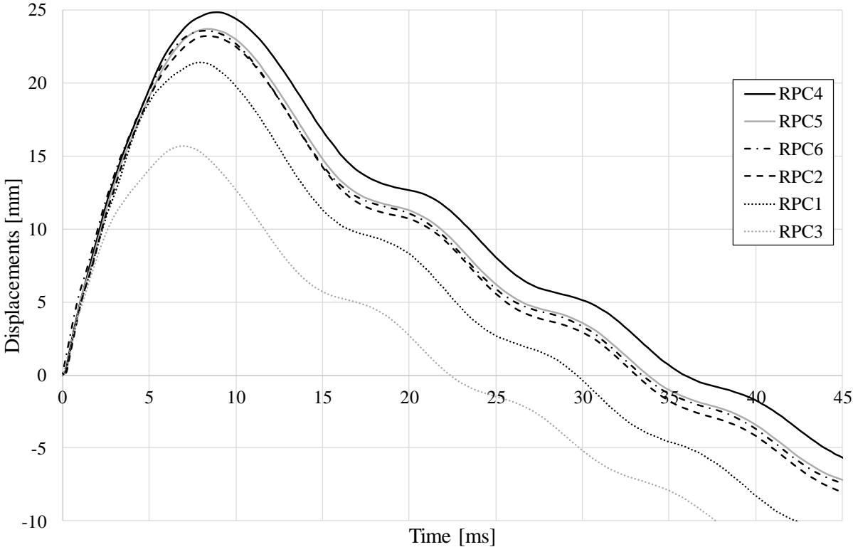
Figure 6.6 Results for the displacement of the midpoint for the beams used in the experiments.
