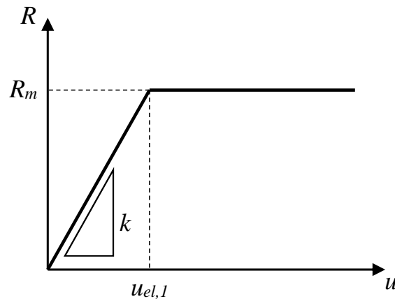
Figure 2.5 The internal resisting force and displacement relation for an elastoplastic material.
