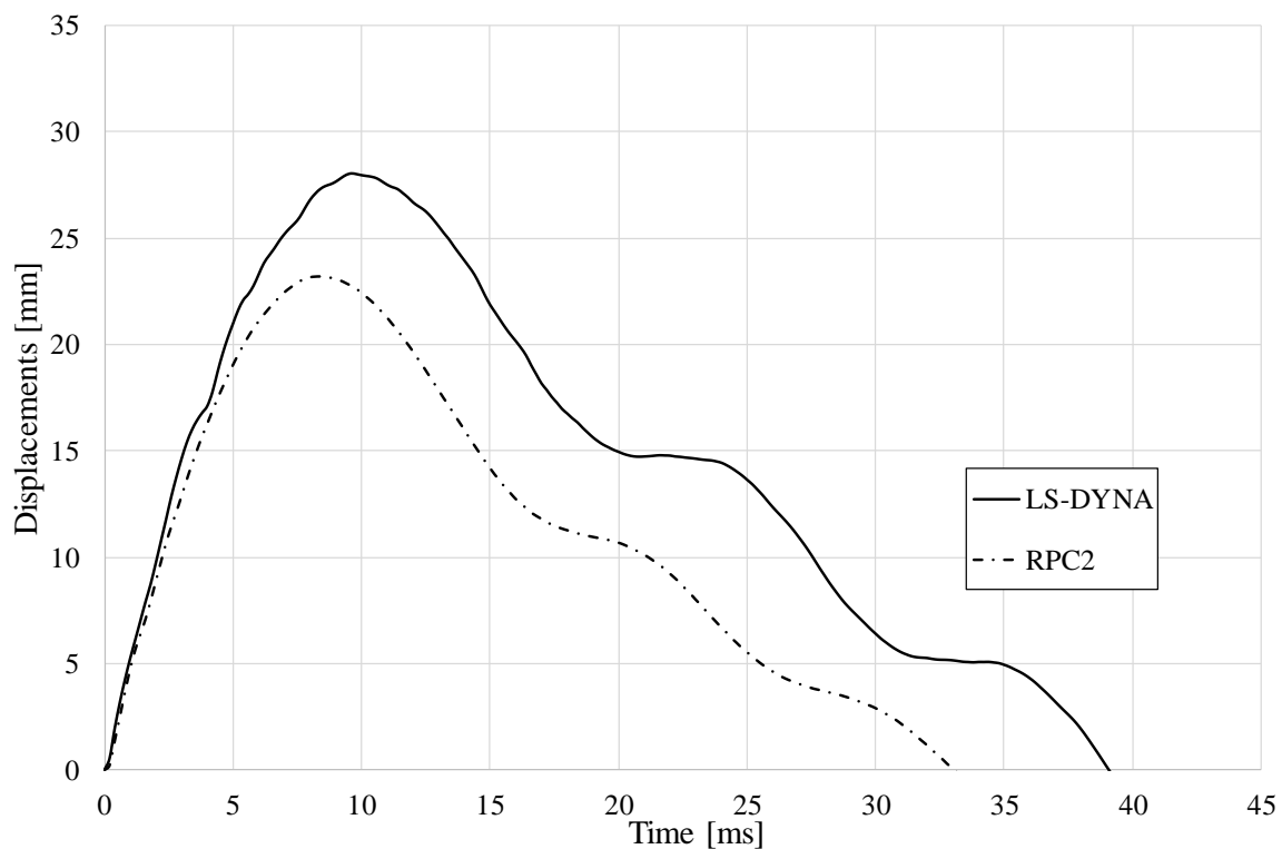
Figure 6.12 Displacement over time for the LS-DYNA model and RPC2, respectively.
