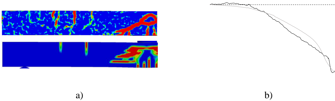
Figure D.29 Response after 0.6 ms: a) Crack pattern for RPC2 and LS-DYNA, respectively and b) Displacement shape for RPC2 (black) and LS-DYNA (grey).
