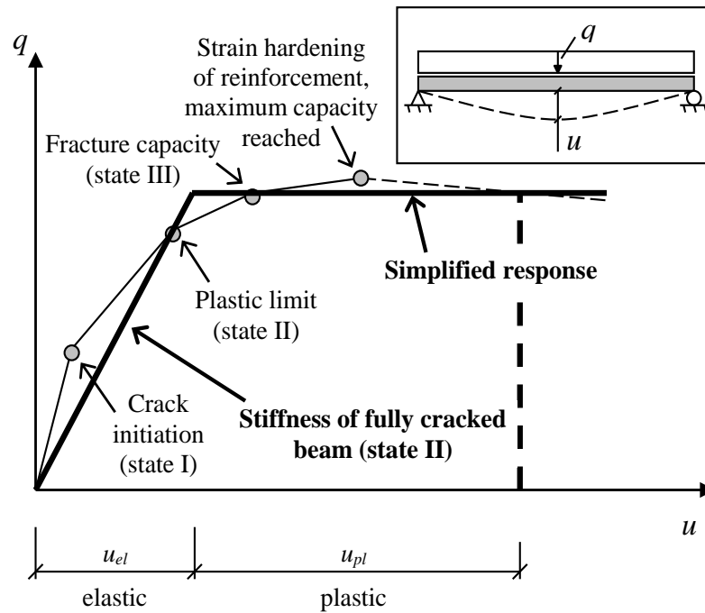
Figure 2.14 Response of a simply supported reinforced concrete beam, based on (Johansson & Laine 2012).
