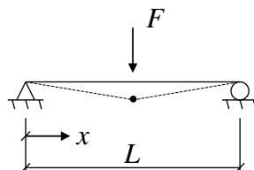
Figure 4.4 Displacement shape of a simply supported beam with a point load at the centre, ideal plastic response.
