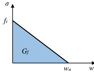
Figure 5.20 A linear damage curve for the CDPM2 material model.
