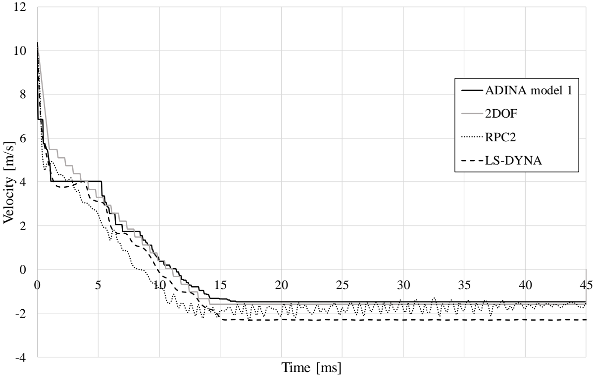
Figure 6.4 Drop weight velocity.
