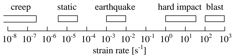
Figure 3.26 Strain rate influence for different load cases. (Johansson 2000)
