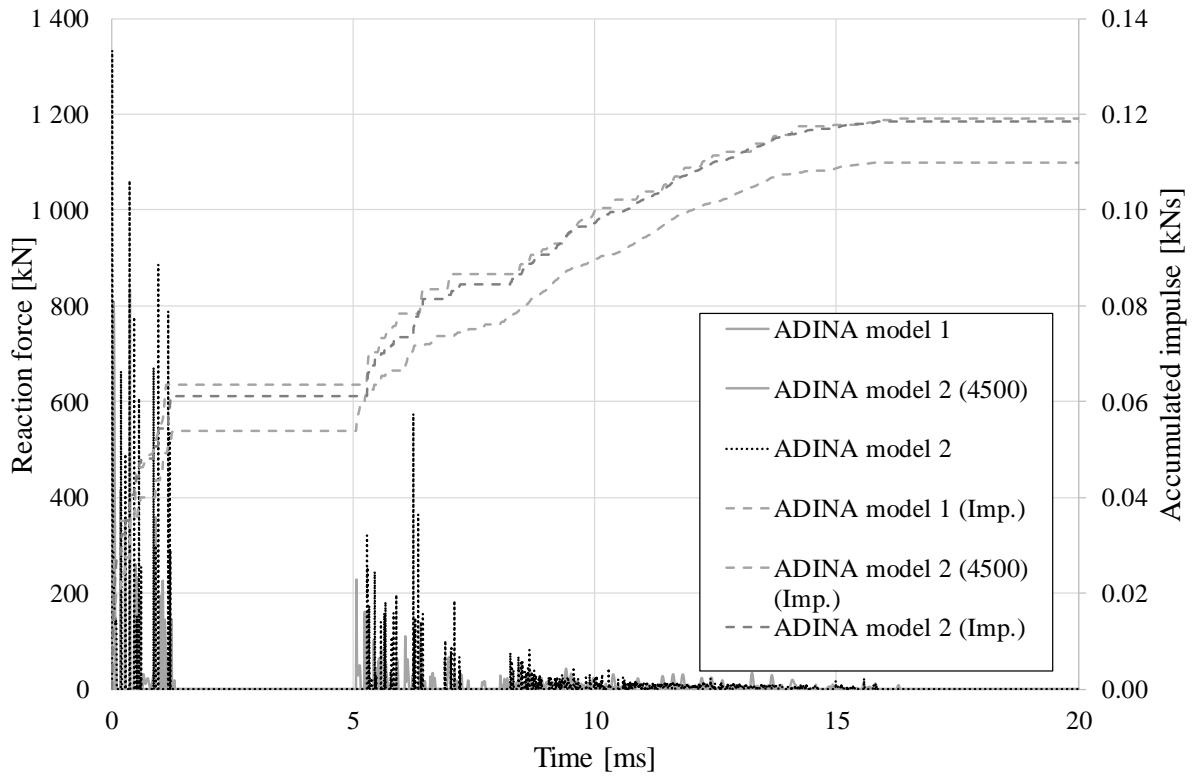
Figure D.9 Reaction force/Accumulated impulse from the drop weight in the ADINA models.
