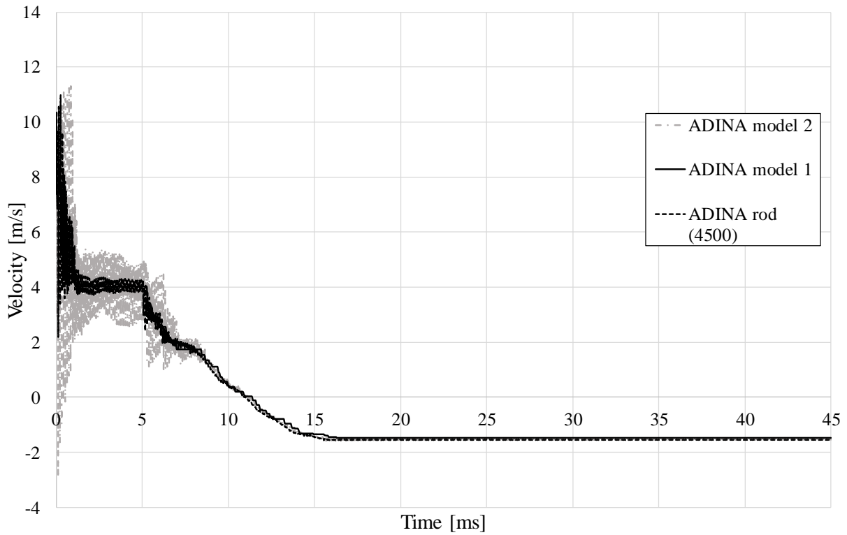
Figure D.7 Drop weight velocity over time for ADINA models.
