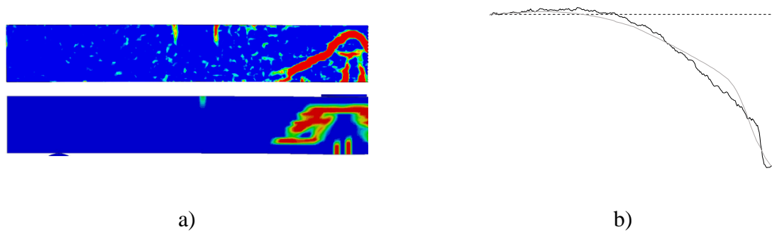
Figure D.28 Response after 0.4 ms: a) Crack pattern for RPC2 and LS-DYNA, respectively and b) Displacement shape for RPC2 (black) and LS-DYNA (grey).
