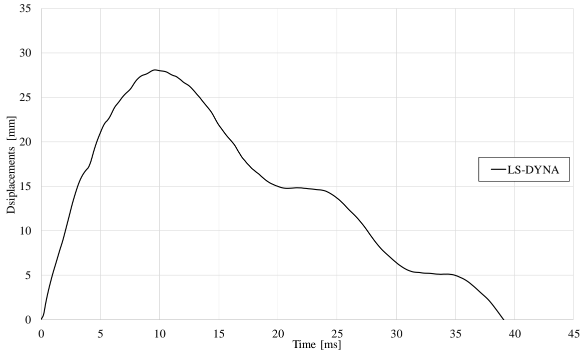
Figure D.12 Midpoint displacement over time of LS-DYNA models.
