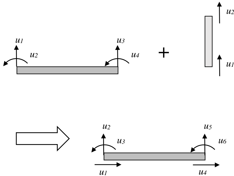
Figure 5.9 Degrees of freedom for a beam element in ADINA.
