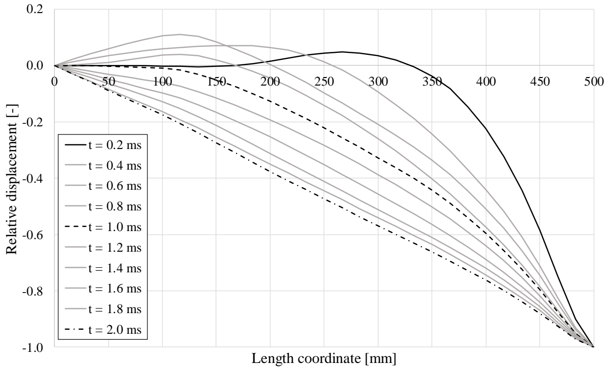
Figure 6.27 Displacement shape of the beam in ADINA model 1 during the first 2 ms.
