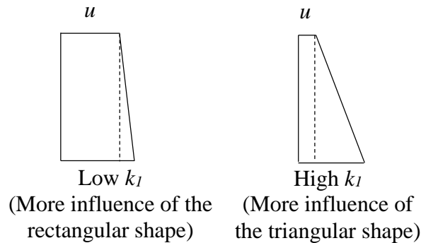
Figure 4.15 Influence on the displacement shapes from the boundary conditions.
