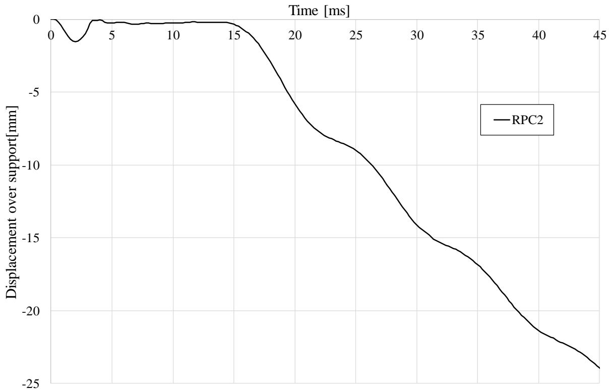
Figure 6.15 Beam displacement by the support over time, where negative displacement represents the beam going in positive y-direction (vertical direction).
