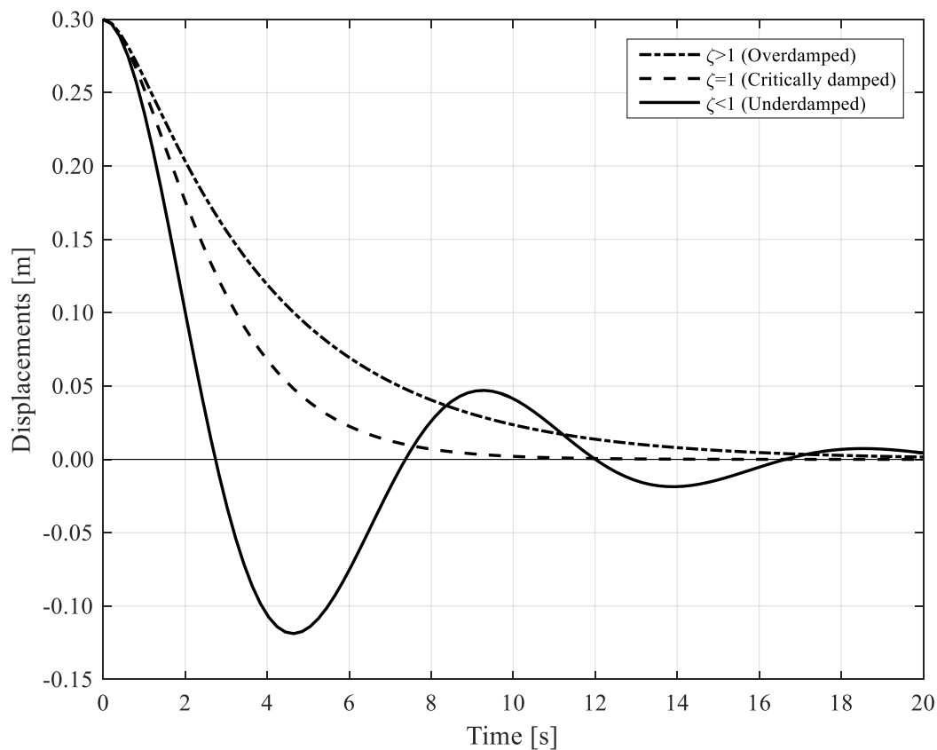
Figure 3.13 Vibration of a damped SDOF system.
