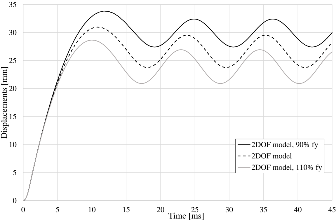
Figure 6.11 Influence of yield strength on the beam response in the 2DOF model.
