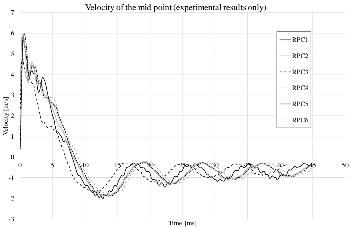
Figure D.23 Midpoint velocity of RPC2.
