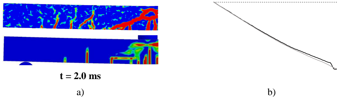
Figure 6.39 Response after 2.0 ms: a) Crack pattern for RPC2 and LS-DYNA, respectively and b) Displacement shape for RPC2 (black) and LS-DYNA (grey).
