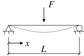
Figure 4.3 Displacement shape of a simply supported beam with a point load at the centre, linear elastic response.
