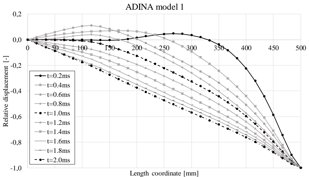
Figure D.4 Displacement over length of ADINA model 1.
