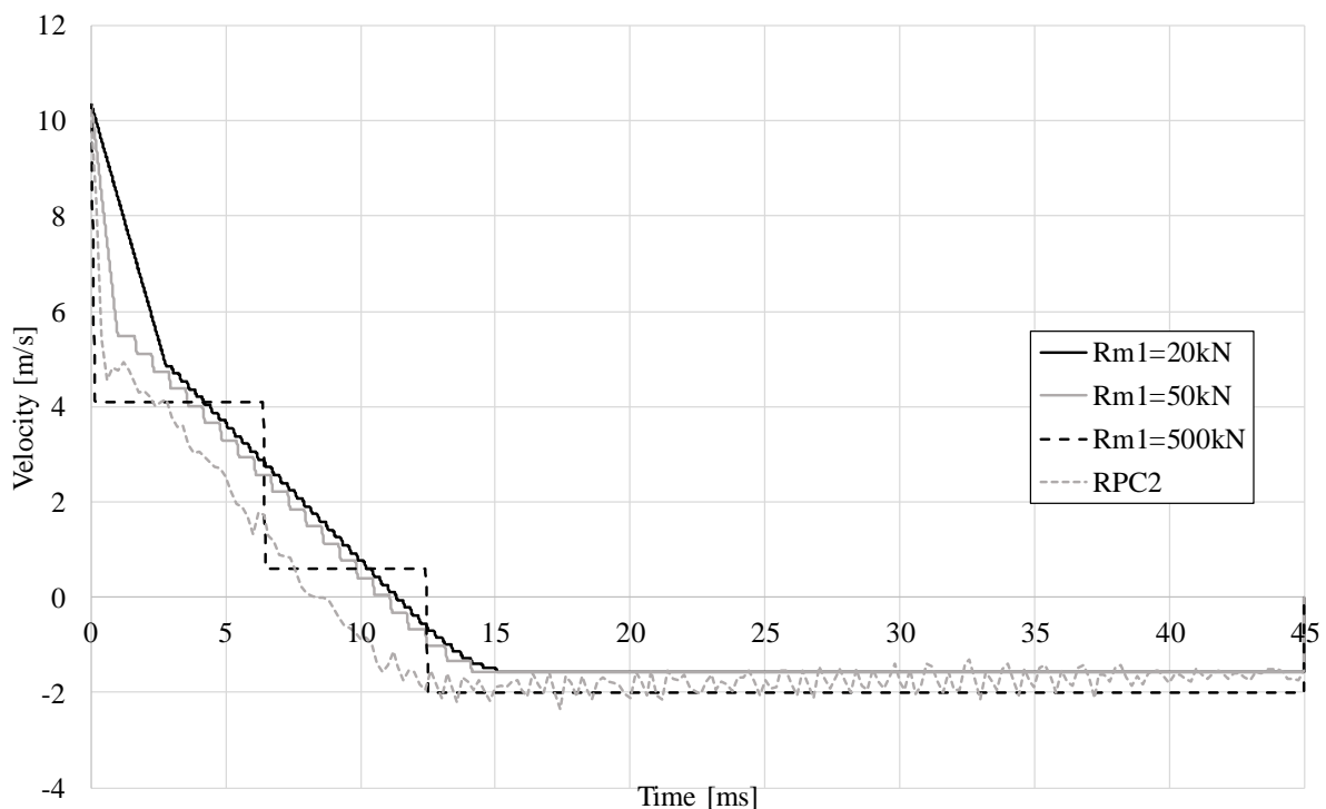
Figure 6.5 Velocity of the drop weight to study of the plastic limit of the 2DOF model.
