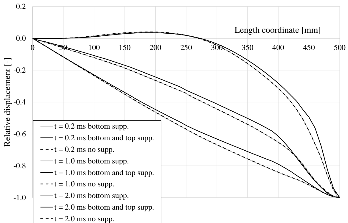
Figure 7.10 Displacement shape u(x) of a LS-DYNA modelled beam with three types of support conditions for three different time steps.
