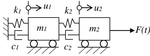
Figure 3.21 2DOF spring-mass system.
