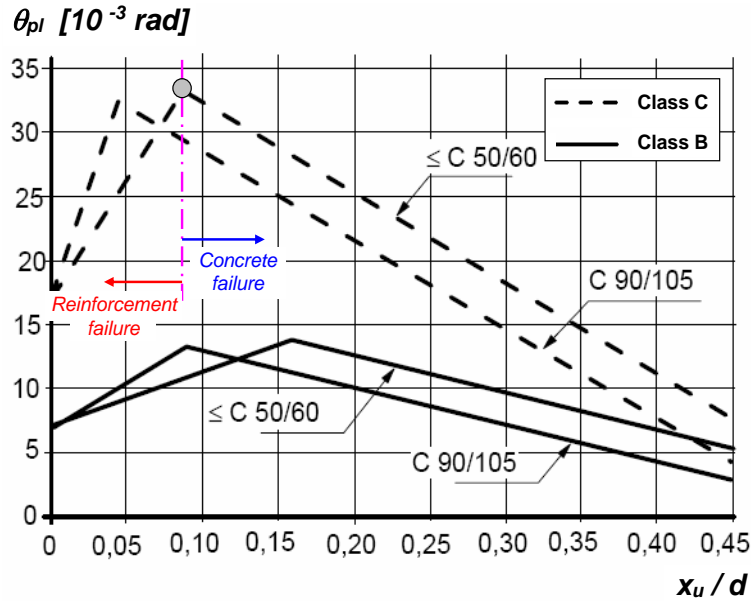
Figure 2.15 Design values for plastic rotation for various concrete and steel types, based on (CEN 2004). The limit between reinforcement failure and concrete failure in the case of concrete class \leq C50/60 and reinforcement class C is shown.
