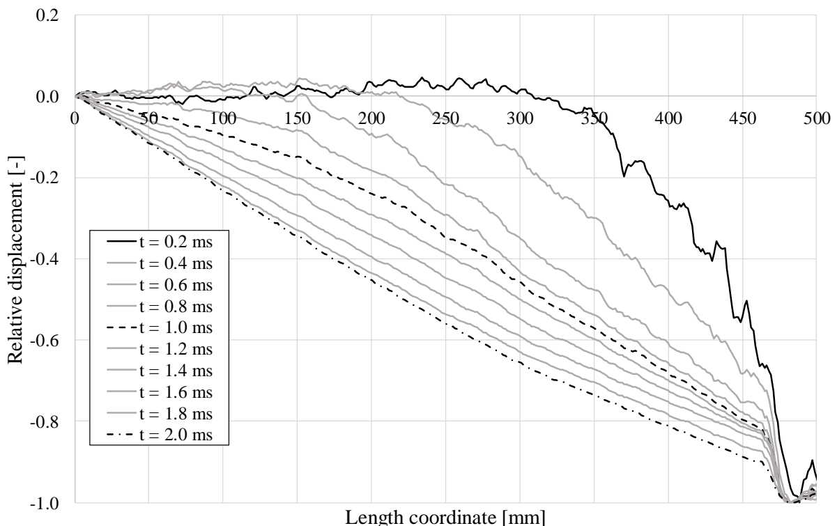
Figure 6.26 Displacement shape of RPC2 during the first 2 ms.
