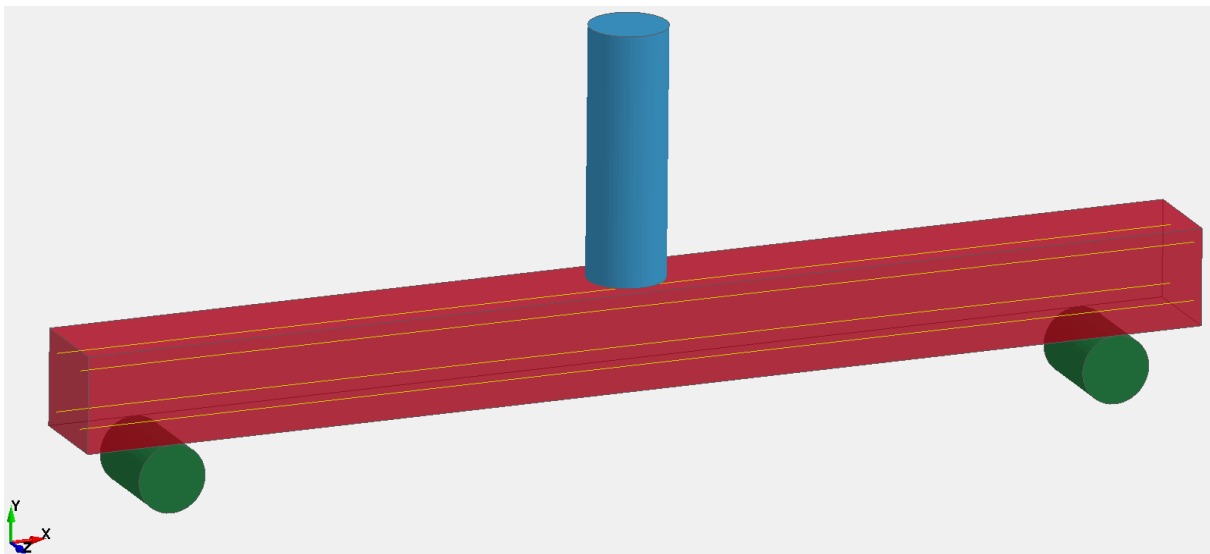
Figure 5.18 LS-DYNA model set up.
