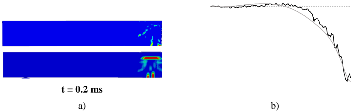
Figure 6.35 Response after 0.2 ms: a) Crack pattern for RPC2 and LS-DYNA, respectively and b) Displacement shape for RPC2 (black) and LS-DYNA (grey).
