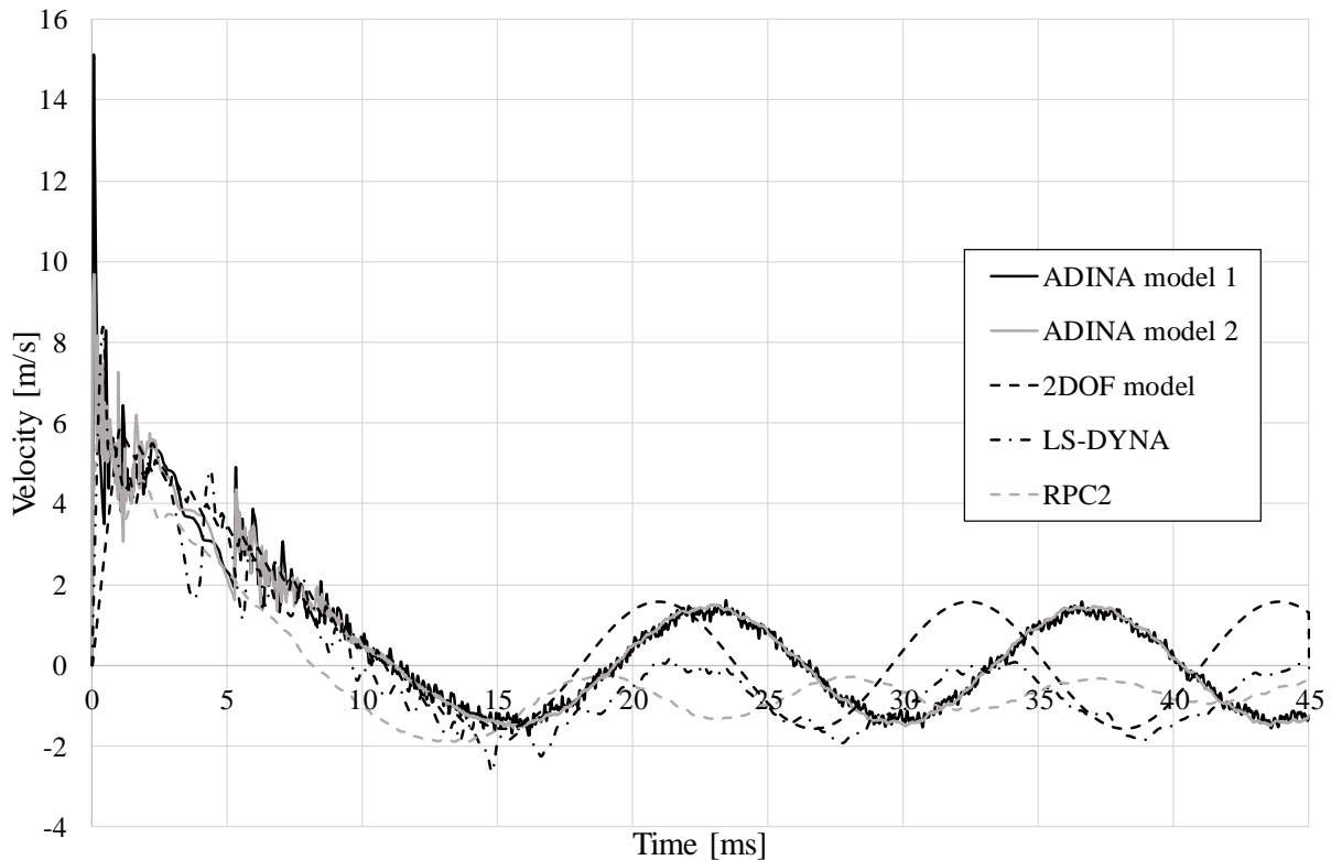
Figure 6.1 Velocity over time for midpoint of the beam.
