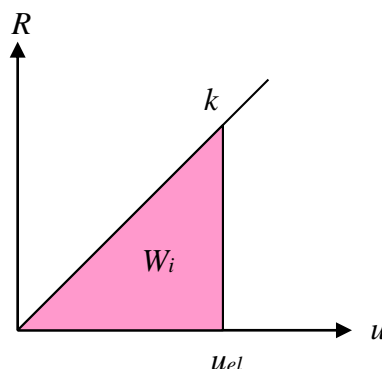
Figure 3.5 Internal work for linear elastic materials.
