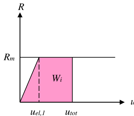
Figure 3.7 Internal work for elastoplastic materials.
