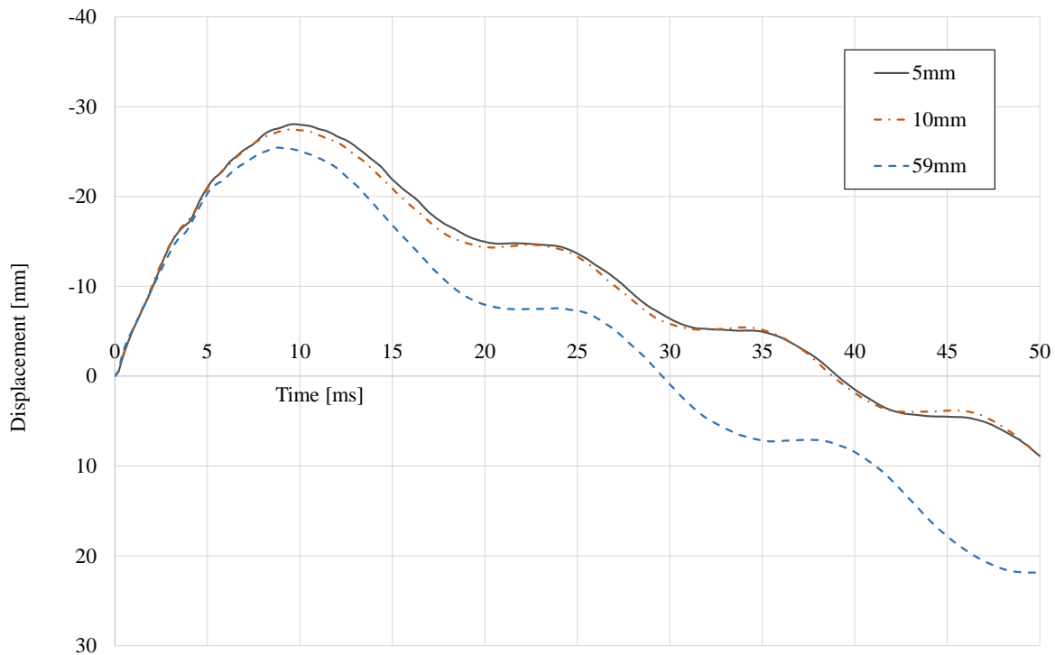
Figure H.5 Displacement of the middle of the beam as a function of time for three different mesh sizes.
