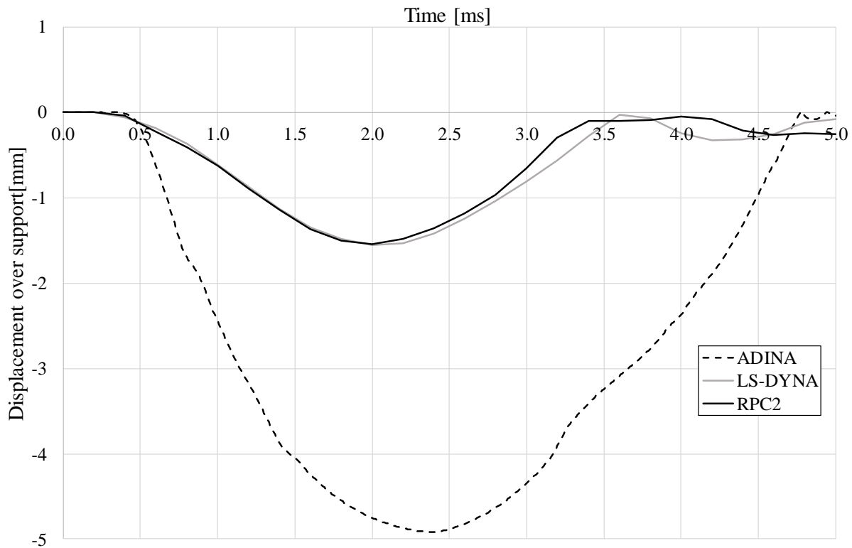
Figure 6.21 Beam displacement over support during the first 4ms.
