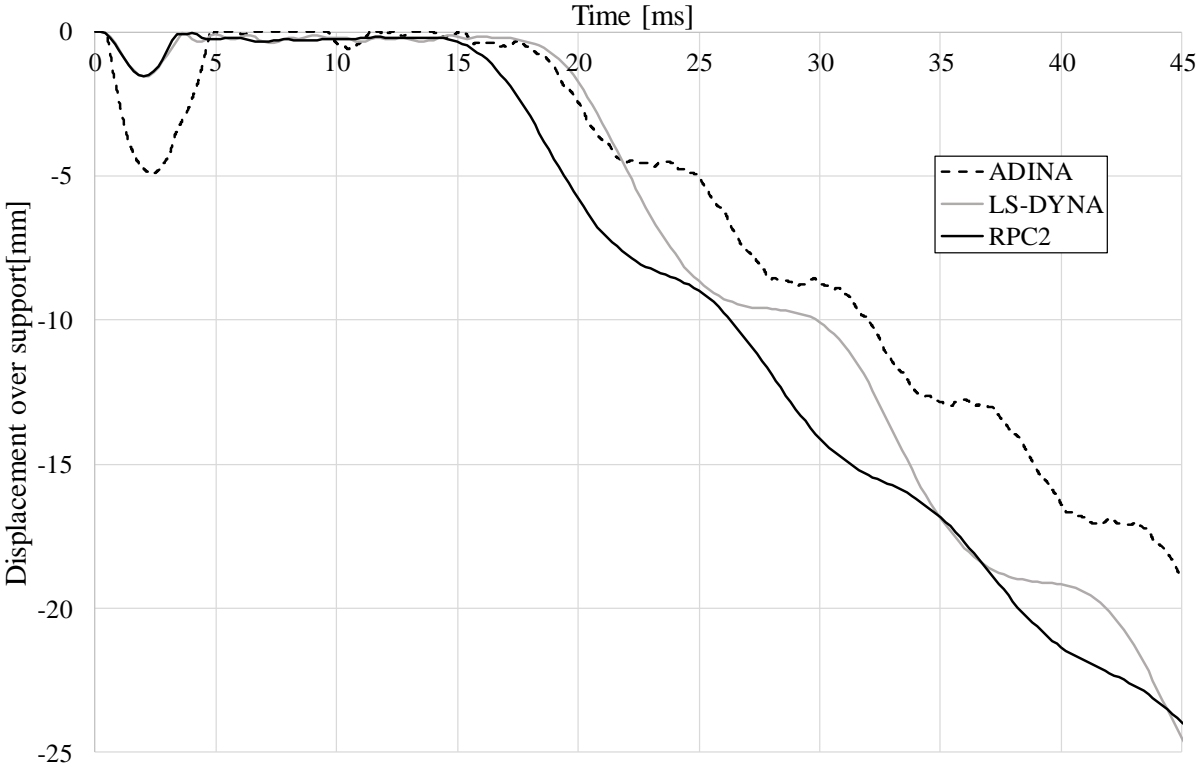
Figure 6.20 Beam displacement over the support over time, results from RPC2, LS-DYNA and ADINA models.
