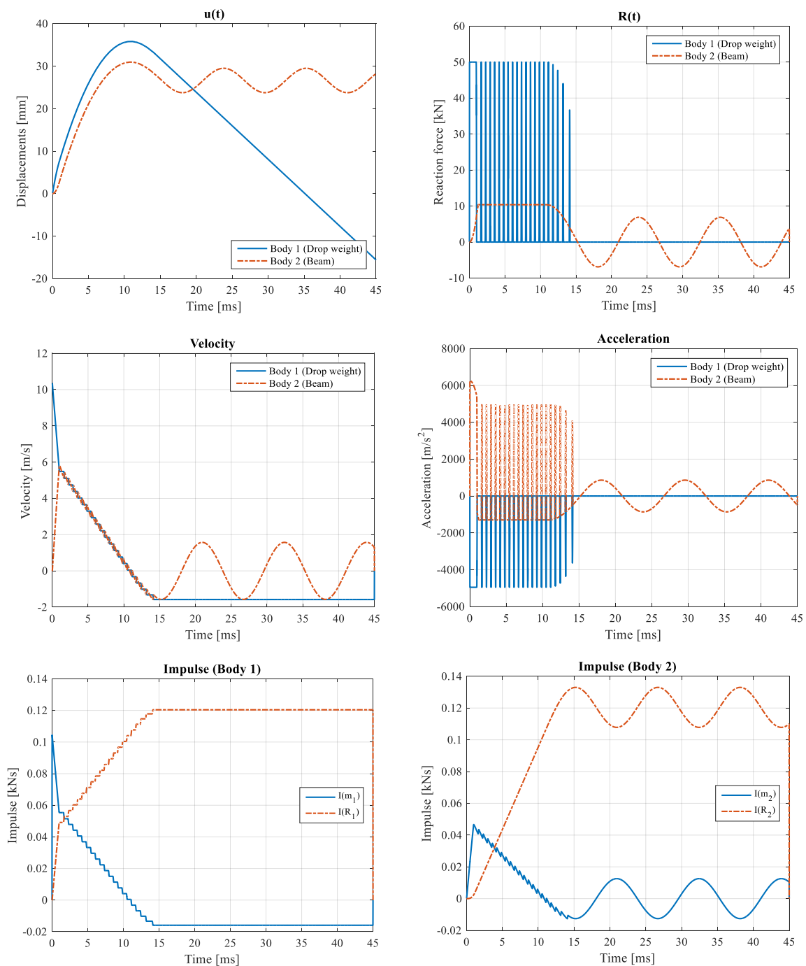
Figure D.1 Results from 2DOF model.
