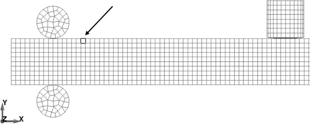
Figure 7.11 Element chosen for stress investigation.
