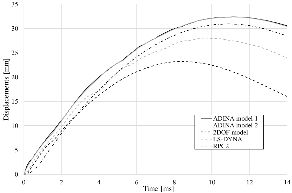
Figure 6.9 Maximum displacement for the analytical models and RPC2 from the experiment.
