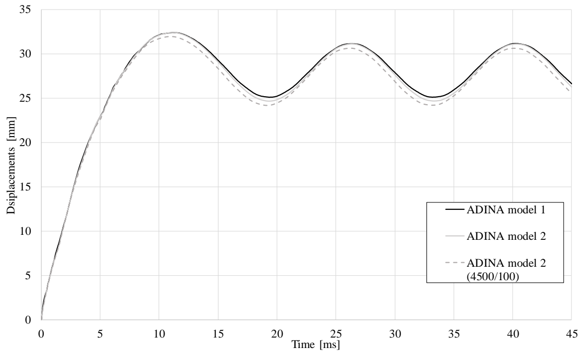
Figure D.3 Midpoint displacement over time of ADINA models.
