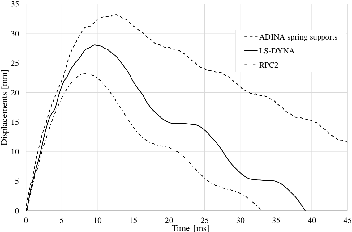
Figure 7.18 Displacement of midpoint over time.
