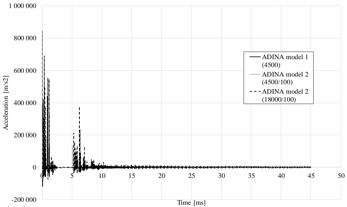
Figure D.8 Midpoint acceleration over time for ADINA models.
