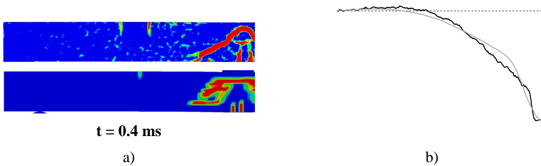
Figure 6.36 Response after 0.4 ms: a) Crack pattern for RPC2 and LS-DYNA, respectively and b) Displacement shape for RPC2 (black) and LS-DYNA (grey).
