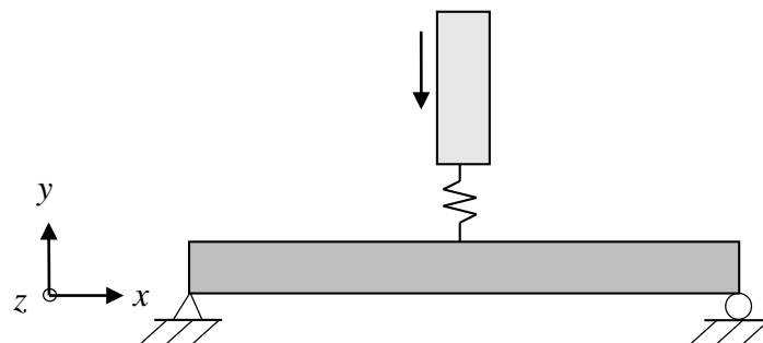
Figure 5.10 Boundary conditions for the FE-models in ADINA.
