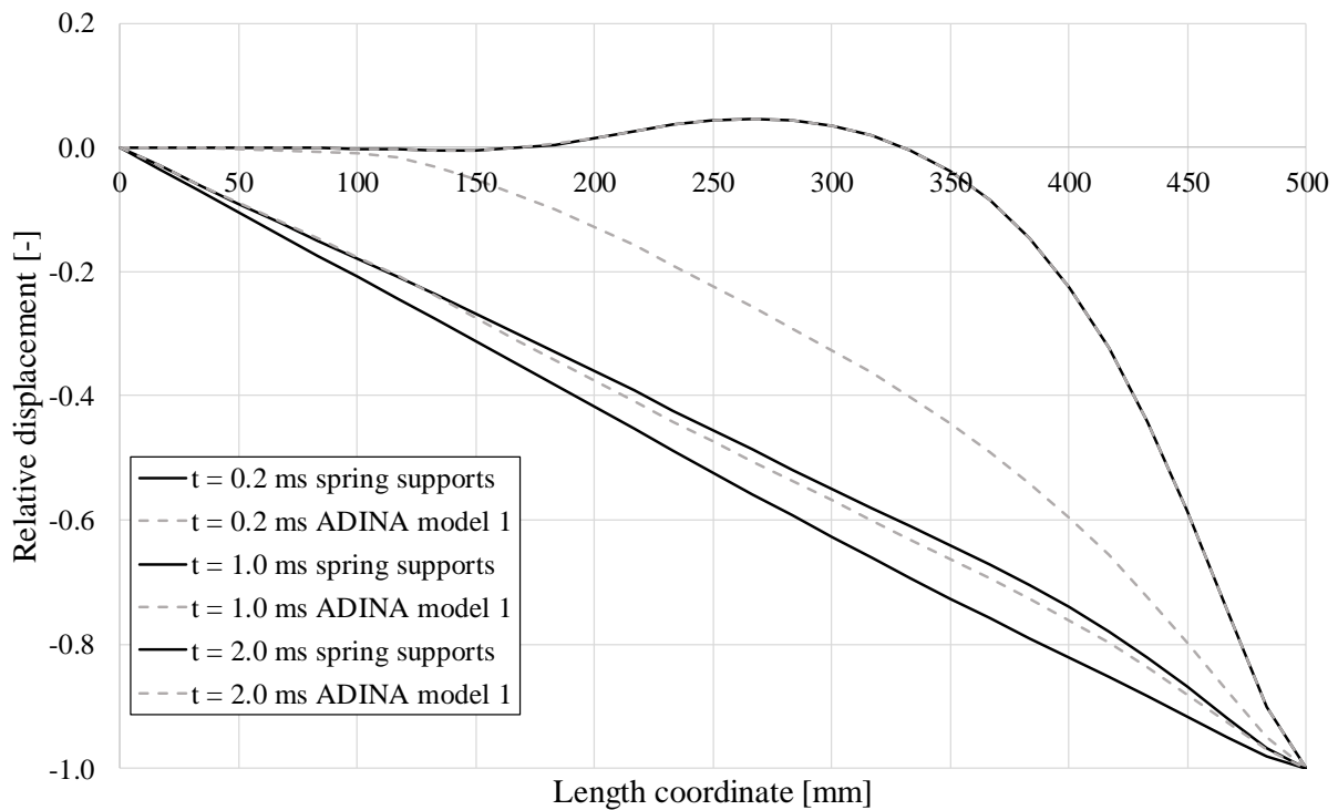
Figure 7.19 Displacement over length of the beam at different times for the model with the spring supports and ADINA model 1, respectively.
