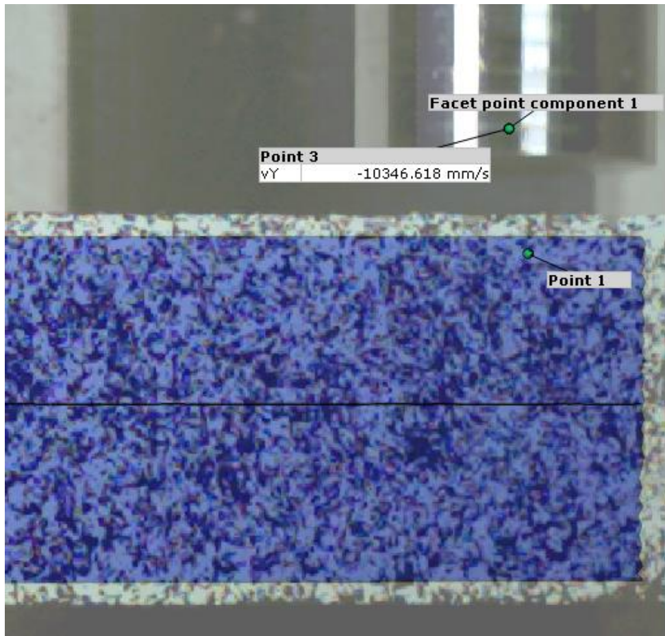
Figure D.25 Part of the experiment showing the drop weight and the beam just before impact when digital image correlation has been made.
