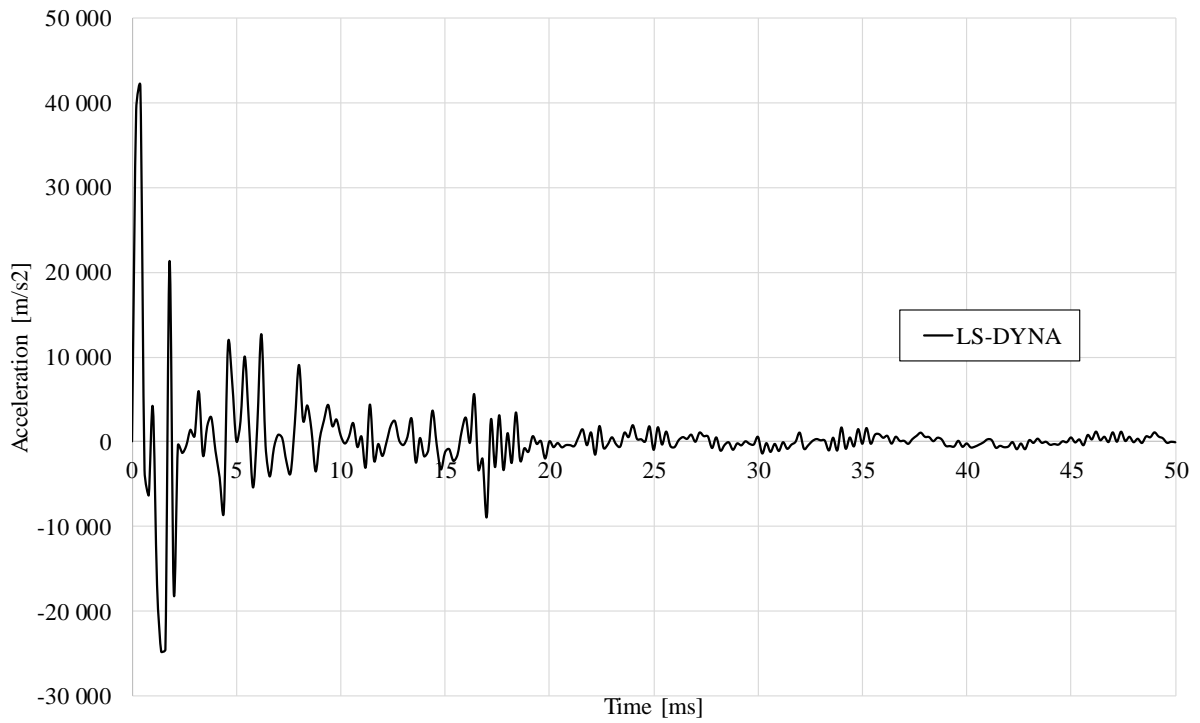
Figure D.18 Acceleration of the midpoint in LS-DYNA model.
