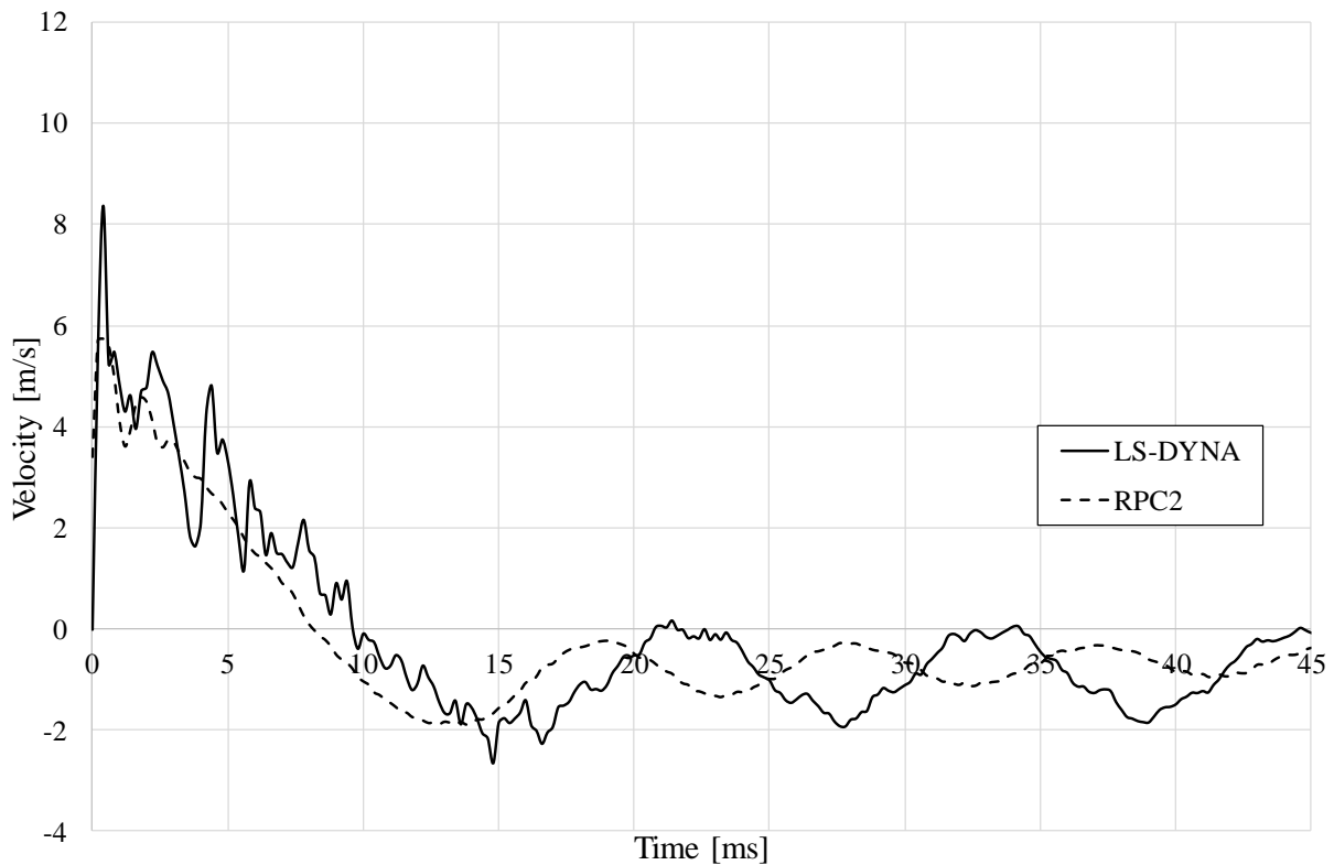
Figure 6.13 Velocity over time of the midpoint for the LS-DYNA model and RPC2.
