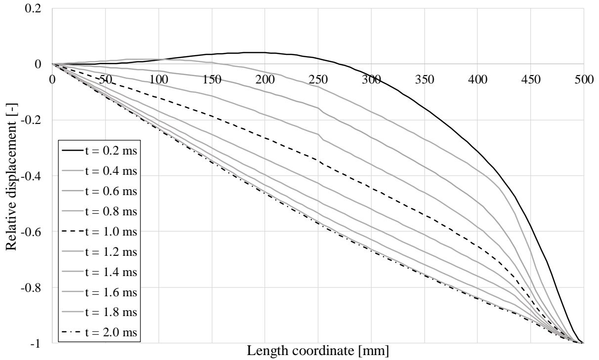
Figure 6.29 Displacement shape of the beam in the LS-DYNA model during the first 2 ms.
