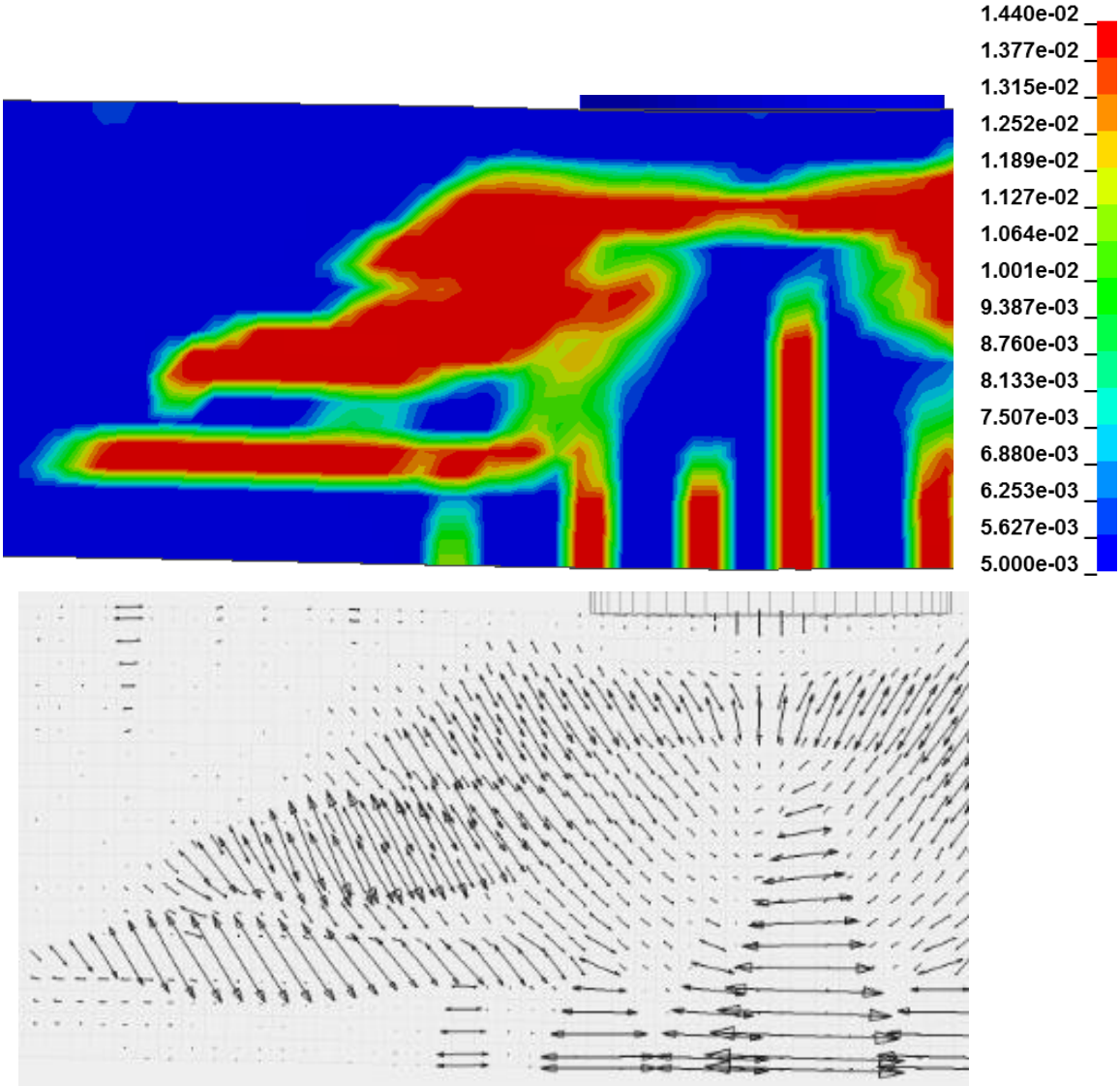
Figure 6.23 1 st principle strain 0.8 ms after impact along with a vector plot showing the direction of the strain for the middle area of the beam.
