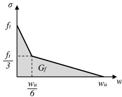
Figure 7.2 Calculated values for a bilinear fracture energy damage model.
