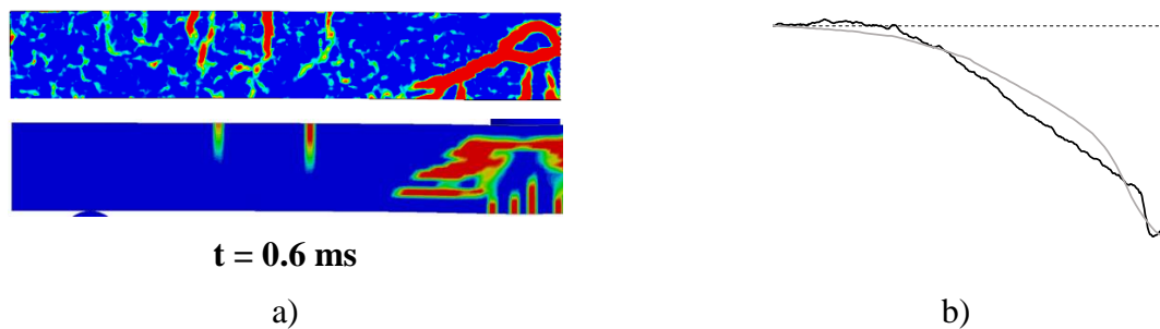
Figure 6.37 Response after 0.6 ms: a) Crack pattern for RPC2 and LS-DYNA, respectively and b) Displacement shape for RPC2 (black) and LS-DYNA (grey).
