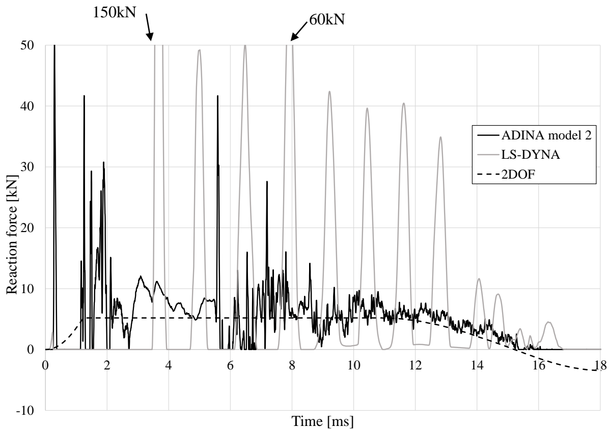
Figure 6.17 Reaction force over supports during the first 15ms, adjusted for lift.
