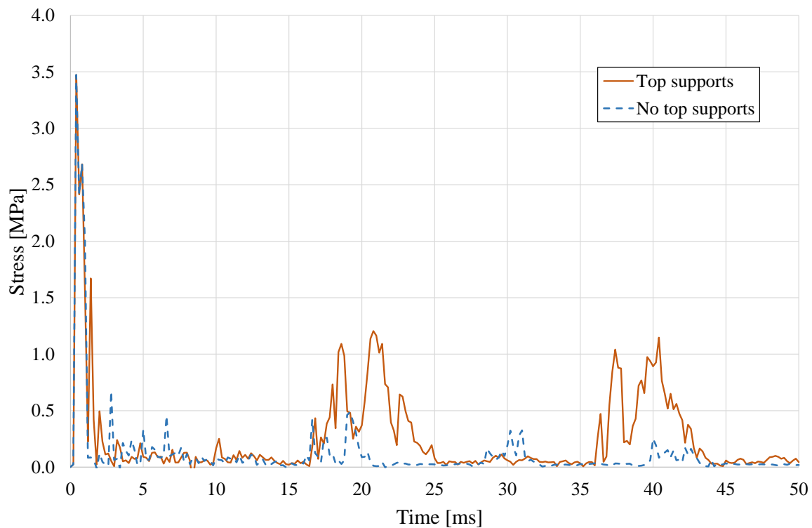
Figure 7.12 Stress in the x -direction in the upper side of the beam as a function of time, shown for both support cases.
