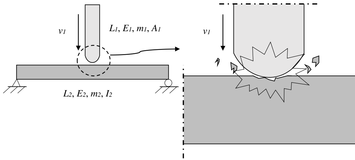
Figure 4.12 The beam-drop weight system and the equivalent transformed mass-spring system.
