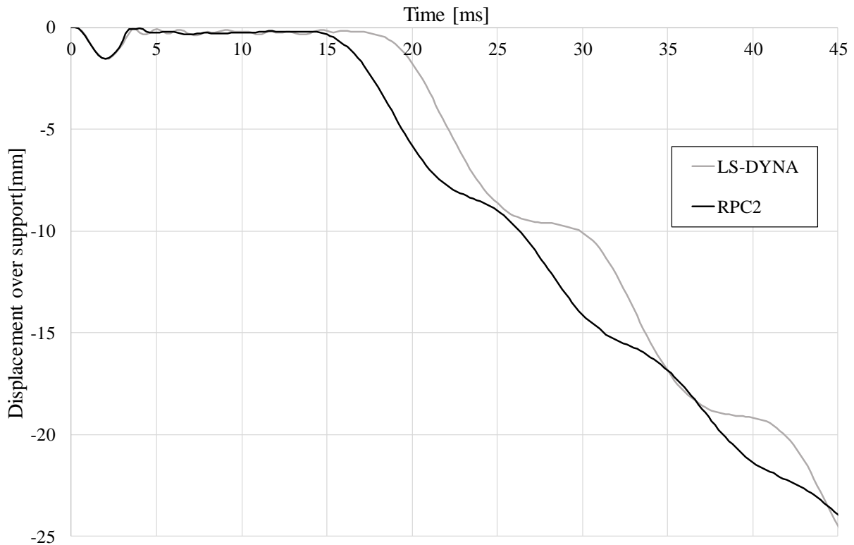
Figure 6.18 Beam displacement over the support over time, results from RPC2 and the LS-DYNA model.
