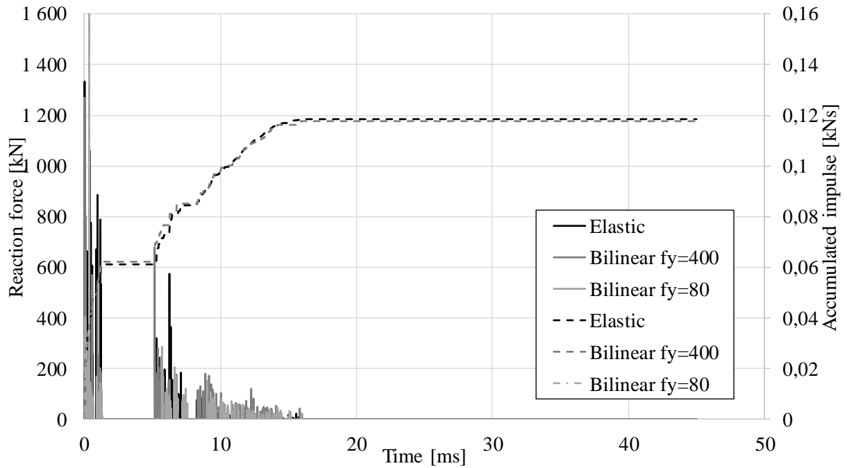
Figure D.11 Comparison elastic/bilinear material response of the drop weight.
