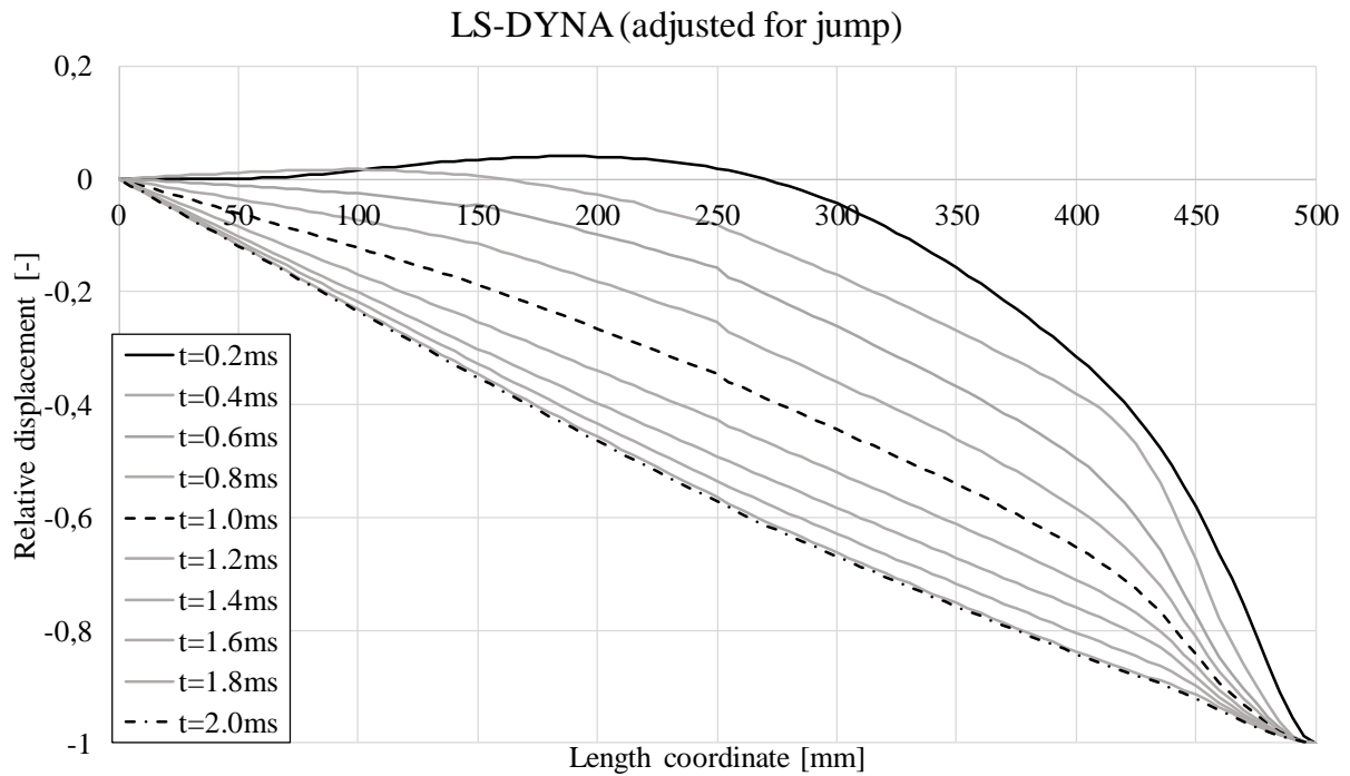
Figure D.14 Displacement over length for LS-DYNA model, adjusted for jump at supports-
