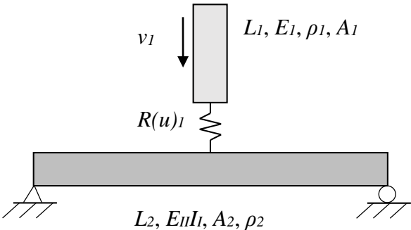
Figure 5.7 The model used in the second ADINA analysis (ADINA model 2), with a rod hitting a beam.
