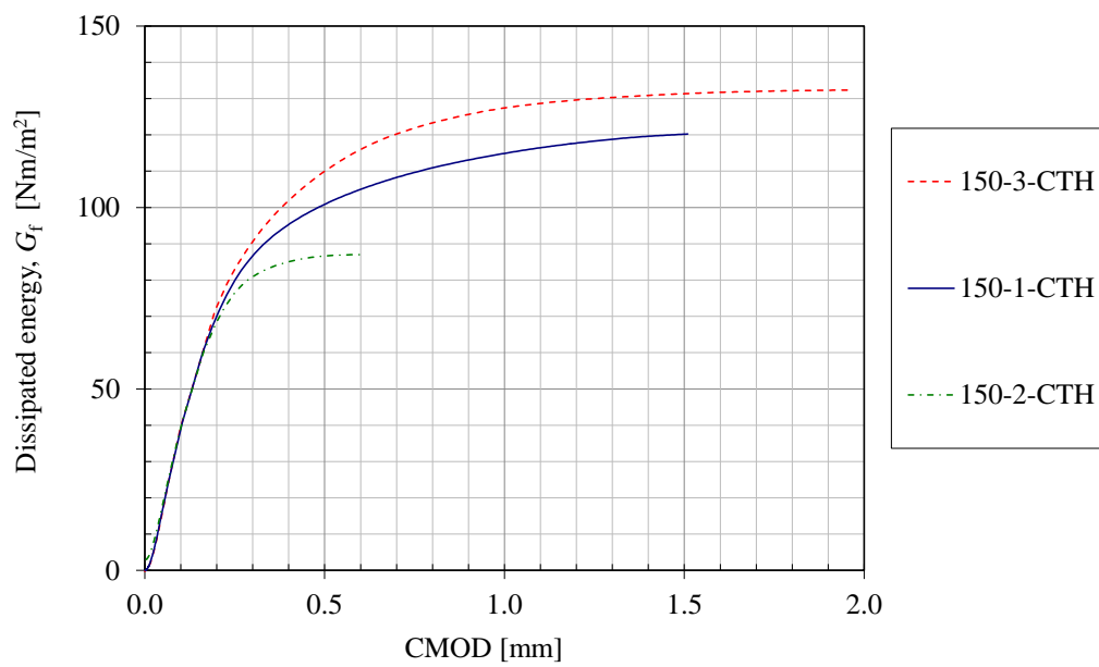
Figure C.1 Accumulated fracture energy measured in three different test specimens.
