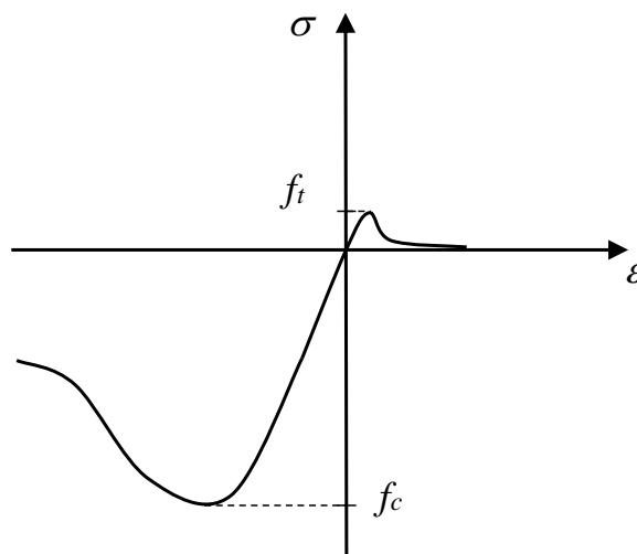
Figure 2.6 Stress-strain relationship for concrete.
