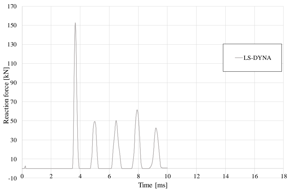
Figure D.20 Reaction force of support for LS-DYNA model during the first 10 ms.
