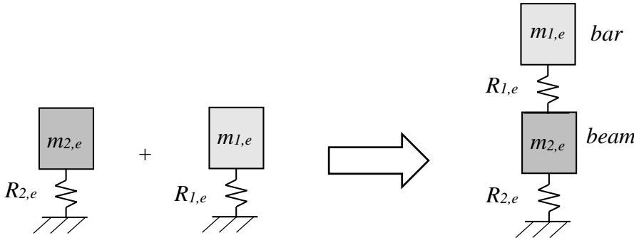
Figure 4.10 Two SDOF system becomes one 2DOF system.
