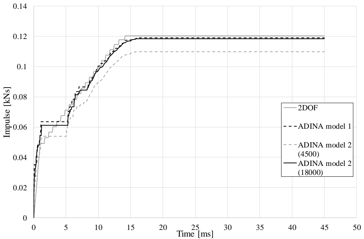
Figure 5.16 Impulse of the load for the different models.
