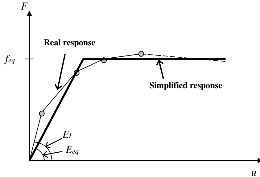
Figure 5.11 Equivalent Young's modulus.
