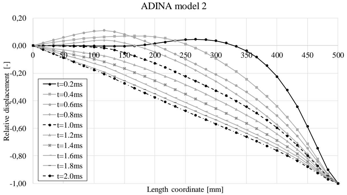
Figure D.5 Displacement over length of ADINA model 2.
