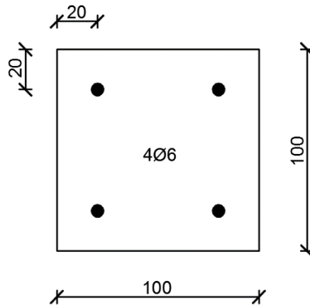
Figure 5.5 Cross section of the concrete beam.
