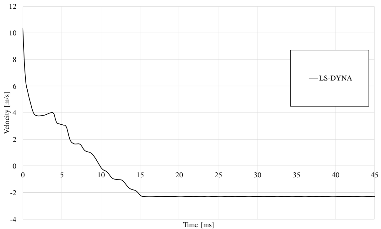
Figure D.17 Velocity of rod in LS-DYNA model.
