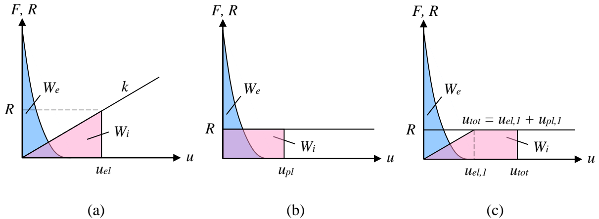
Figure 3.17 Energy equilibrium between external work W_e and internal work W_i for a system with: (a) elastic response, (b) plastic response, (c) elastoplastic response. (Johansson & Laine 2012).
