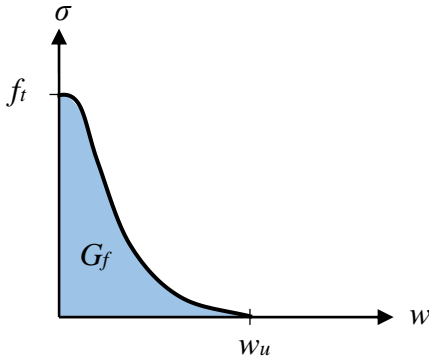
Figure 2.12 Internal work for elastoplastic materials, where w_u is the maximum crack width when the stress reaches zero.
