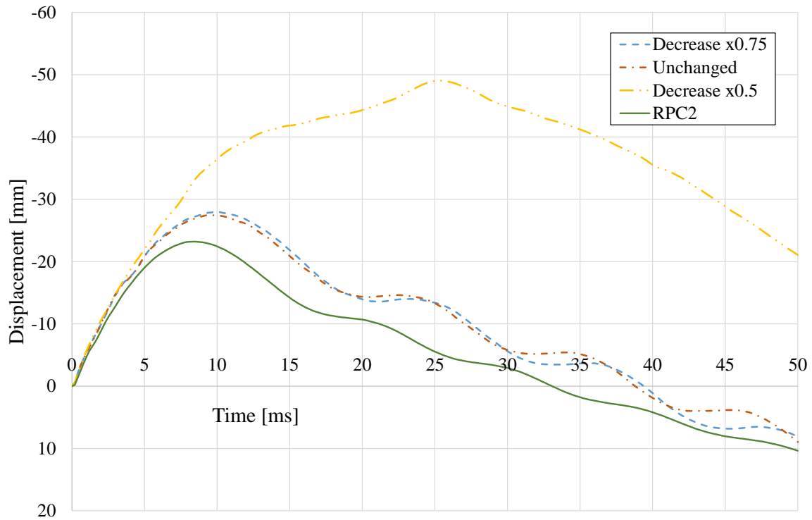
Figure H.7 The midpoint displacement for three values of fracture energy along with the RPC2 test result.
