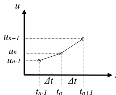
Figure 3.24 Central difference scheme, based on (Carlsson & Kristensson 2012).
