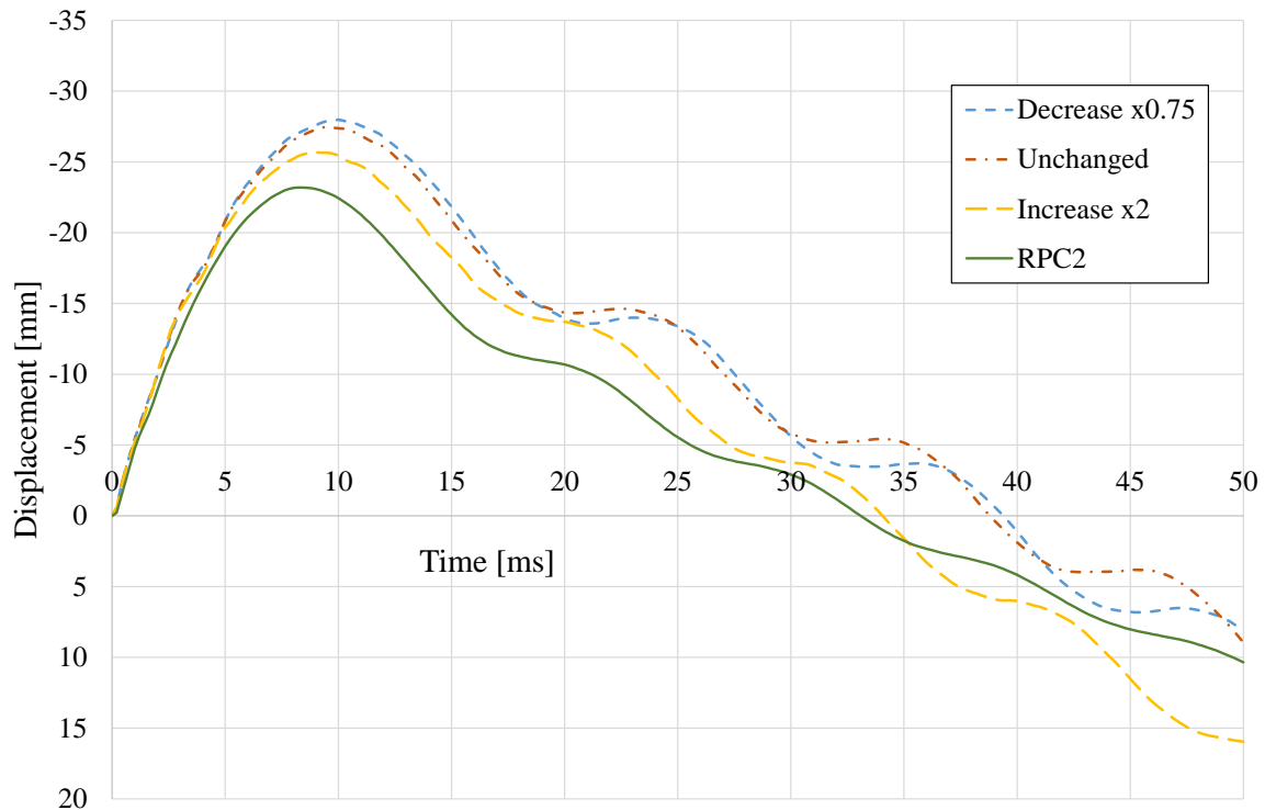
Figure 7.4 Displacement as a function of time for three different magnitudes of fracture energy.
