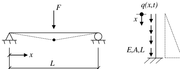
Figure 4.9 Displacement shape of a simply supported beam with ideal plastic response and the response of a bar.
