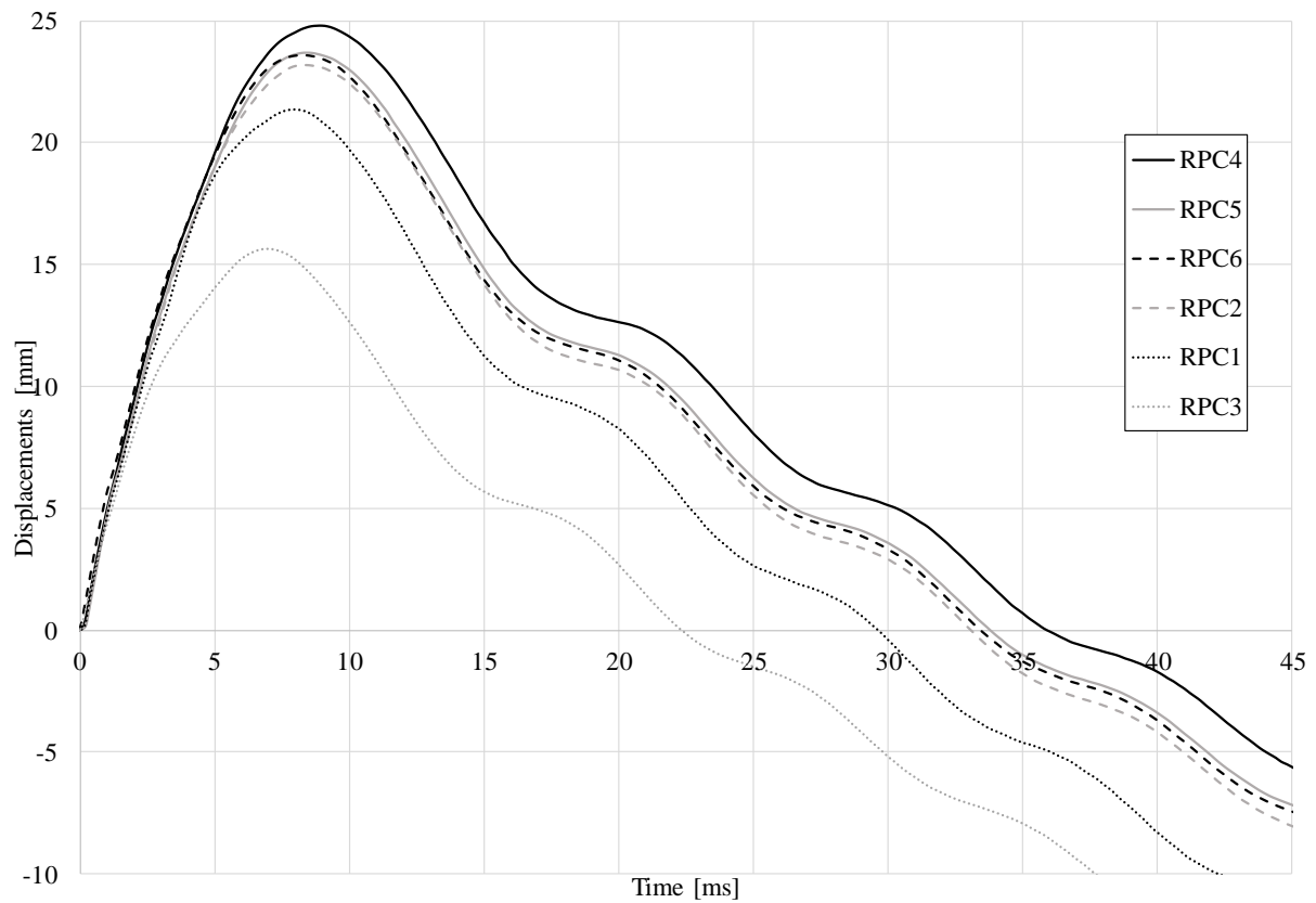
Figure D.21 Midpoint displacement over time from experiment.
