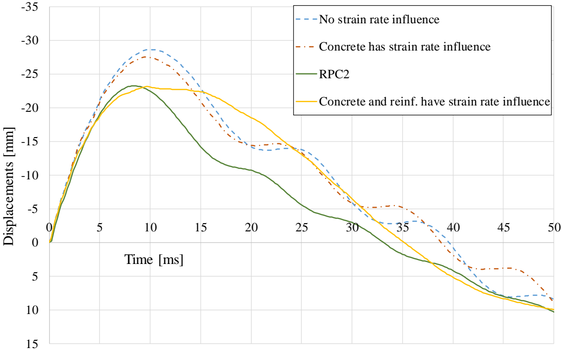
Figure 7.13 Displacement of midpoint as a function of time when strain rate influence was included and excluded in the material models, along with RPC2 test result.
