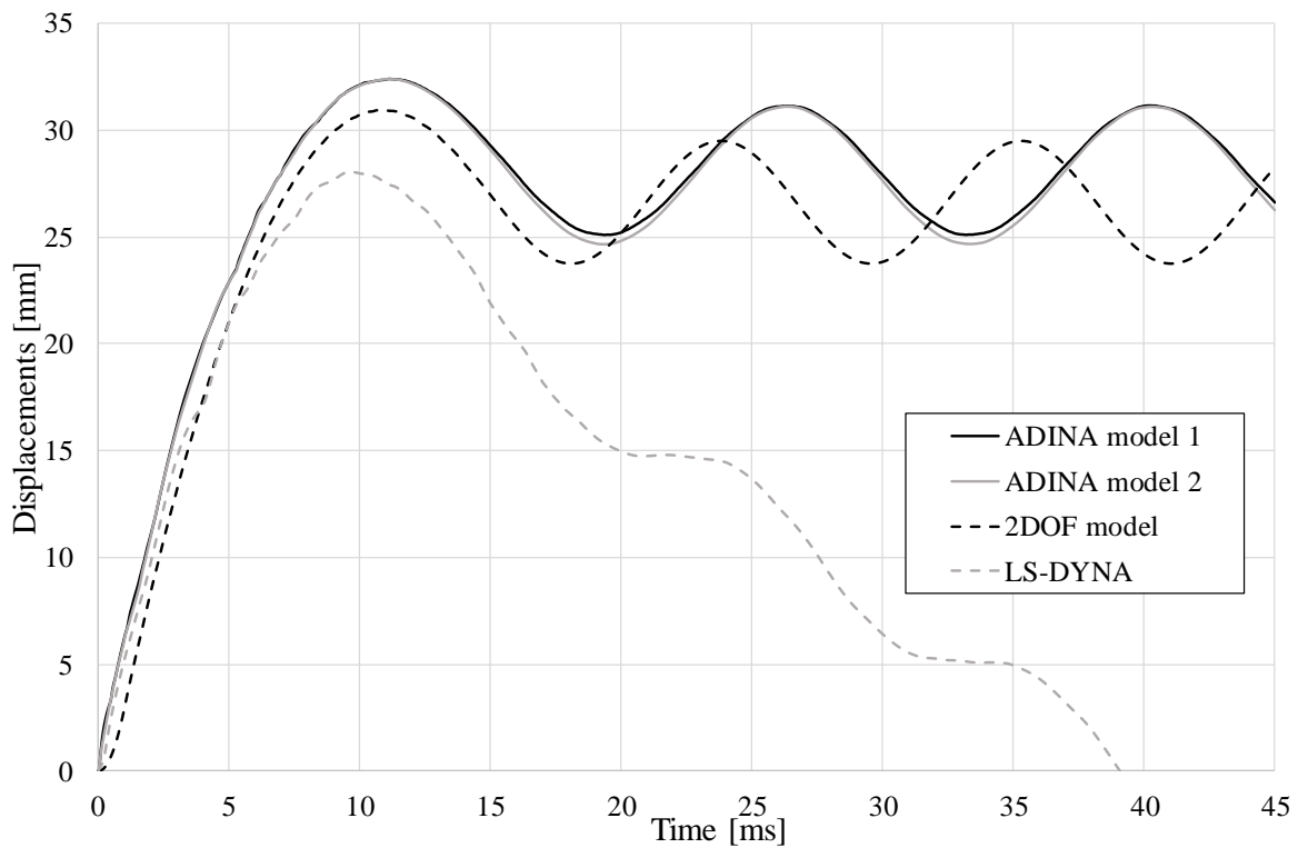
Figure 6.8 Displacement of the midpoint from the different analytical models.
