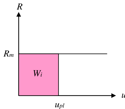
Figure 3.6 Internal work for ideal plastic materials.
