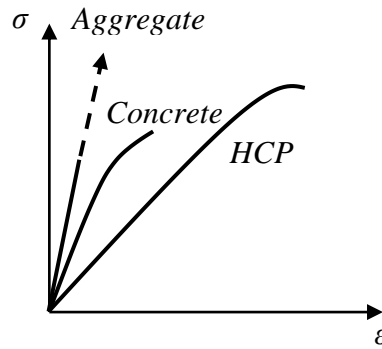
Figure 2.7 Stress-strain relation of aggregates, HCP and concrete as shown in (Domone & Illston 2010)
