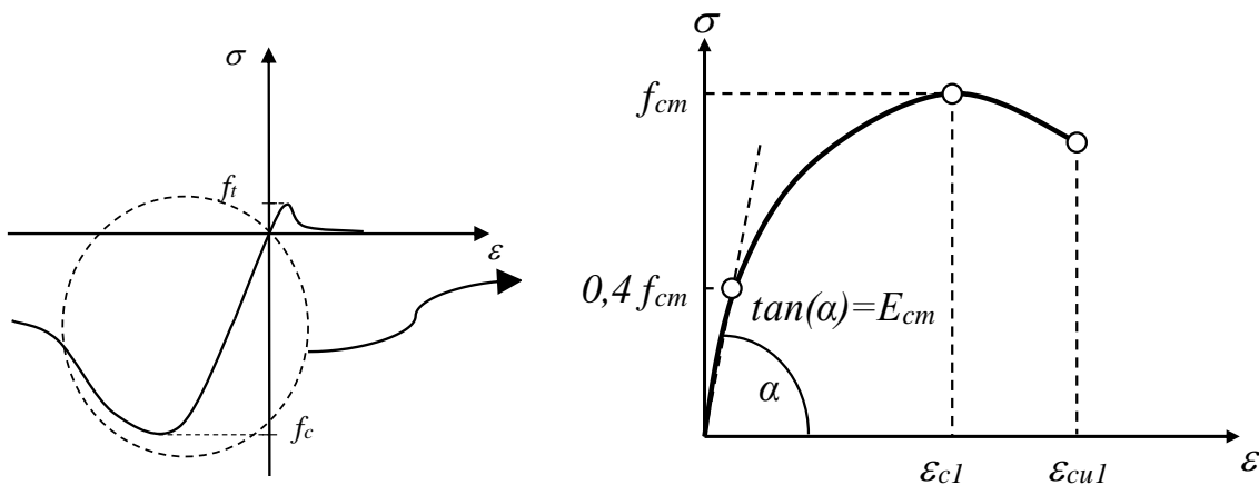
Figure 2.8 Stress-strain relation of concrete in compression for structural analysis.
