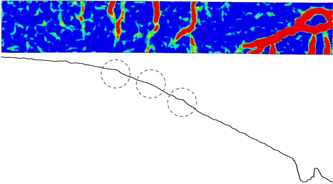
Figure 6.40 Crack pattern/displacement shape for RPC2 after 0.8 ms, with the distinct curvature shifts, at the places where the top cracks appeared.
