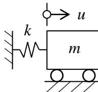
Figure 3.10 Undamped spring-mass system.
