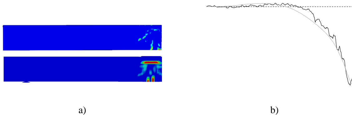
Figure D.27 Response after 0.2 ms: a) Crack pattern for RPC2 and LS-DYNA, respectively and b) Displacement shape for RPC2 (black) and LS-DYNA (grey).
