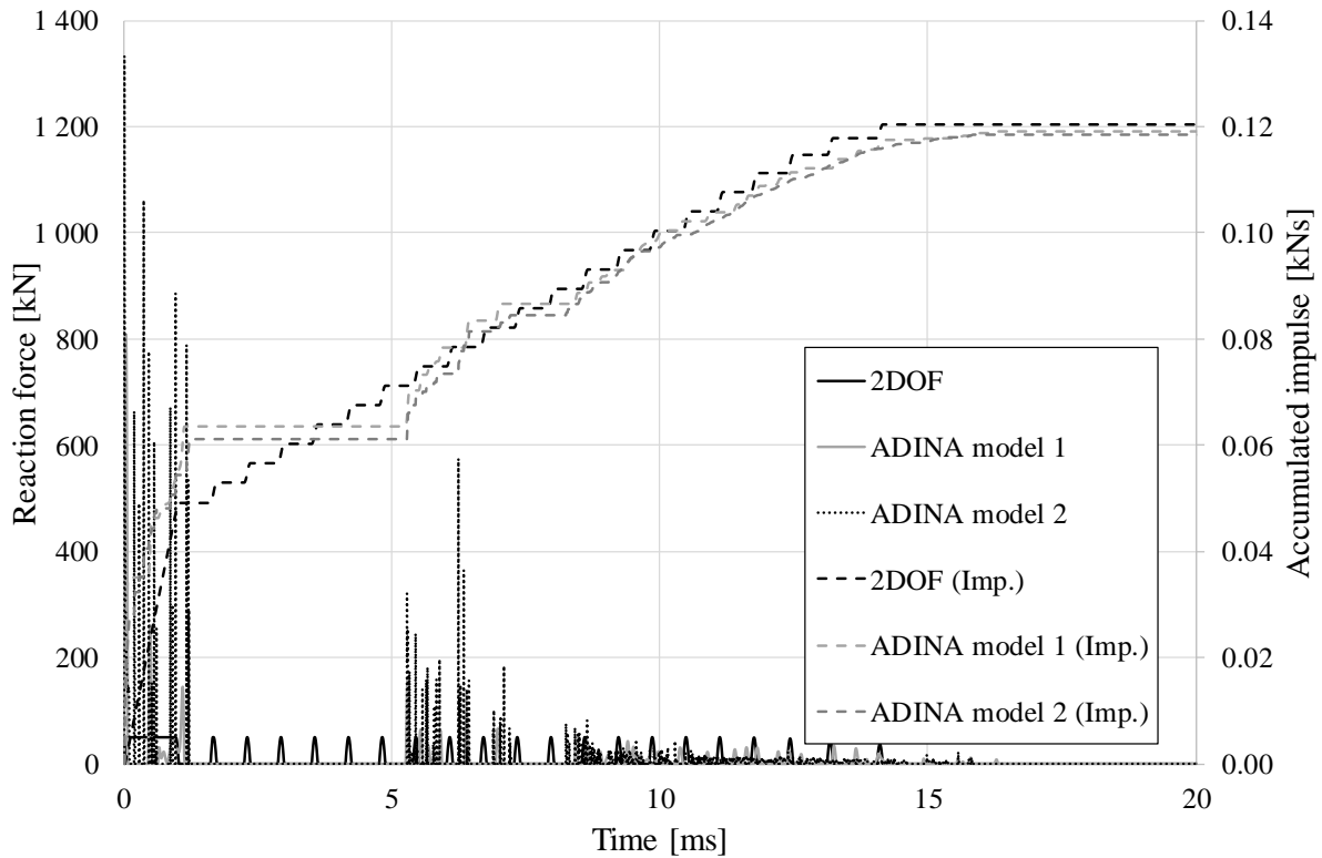
Figure 5.17 Reaction force/accumulated impulse over time.
