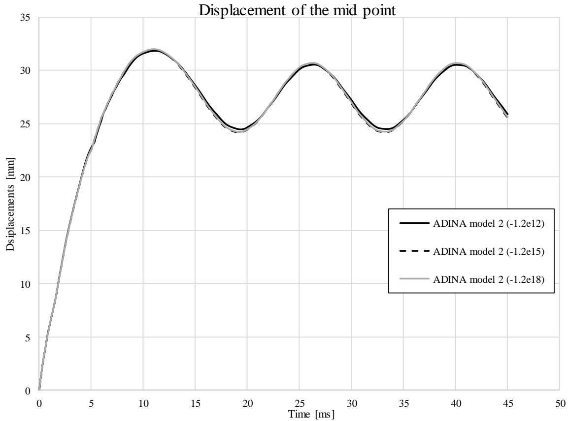
Figure H.2 Response of midpoint using different spring stiffness for ADINA model 2.
