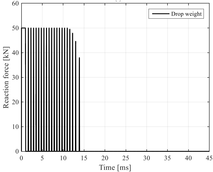
Figure 5.14 Reaction force of the drop weight, used to get an estimation of the load duration. The figure is extracted from the 2DOF model.
