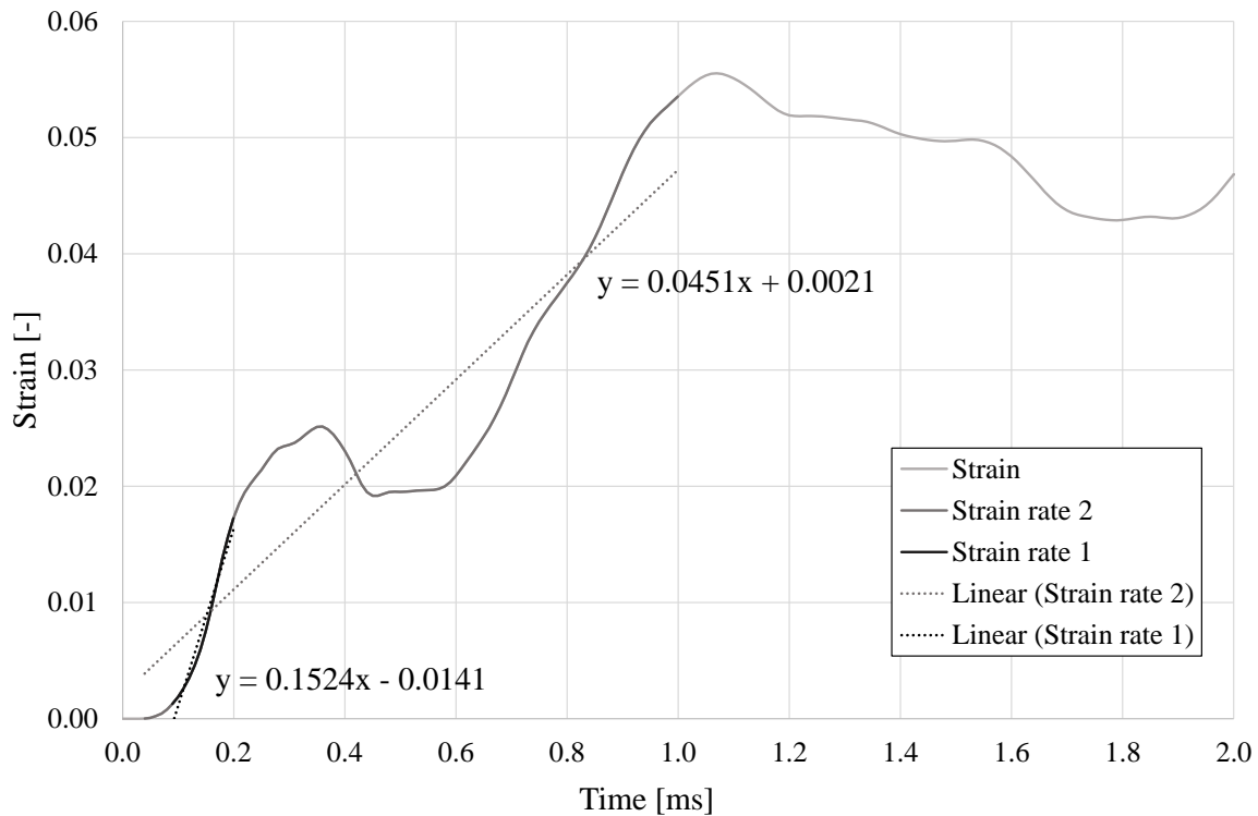
Figure H.6 Strain as a function of time for an element where a bending crack was initiated.
