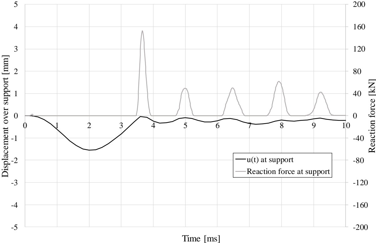
Figure 6.31 Displacement over support/Reaction force of support during the first 10 ms from the LS-DYNA results.
