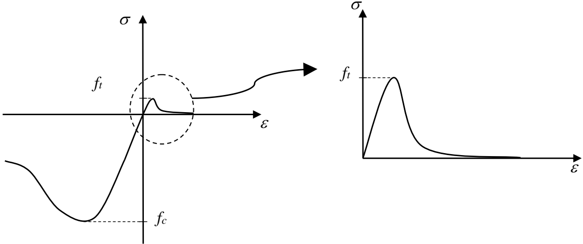
Figure 2.11 Stress strain relationship for concrete in tension
