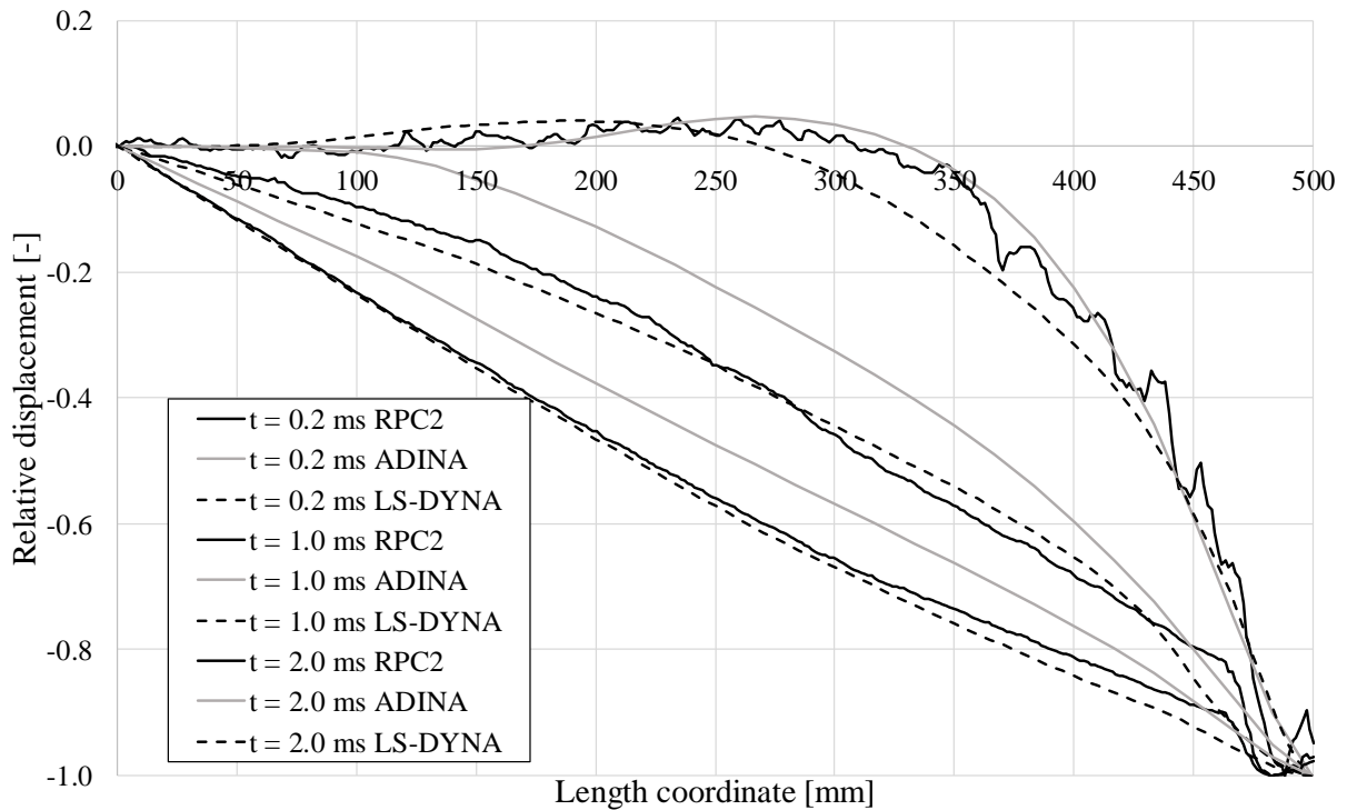
Figure 6.30 Comparison of the displacement shapes of the experimental beam and the numerical models at chosen times.
