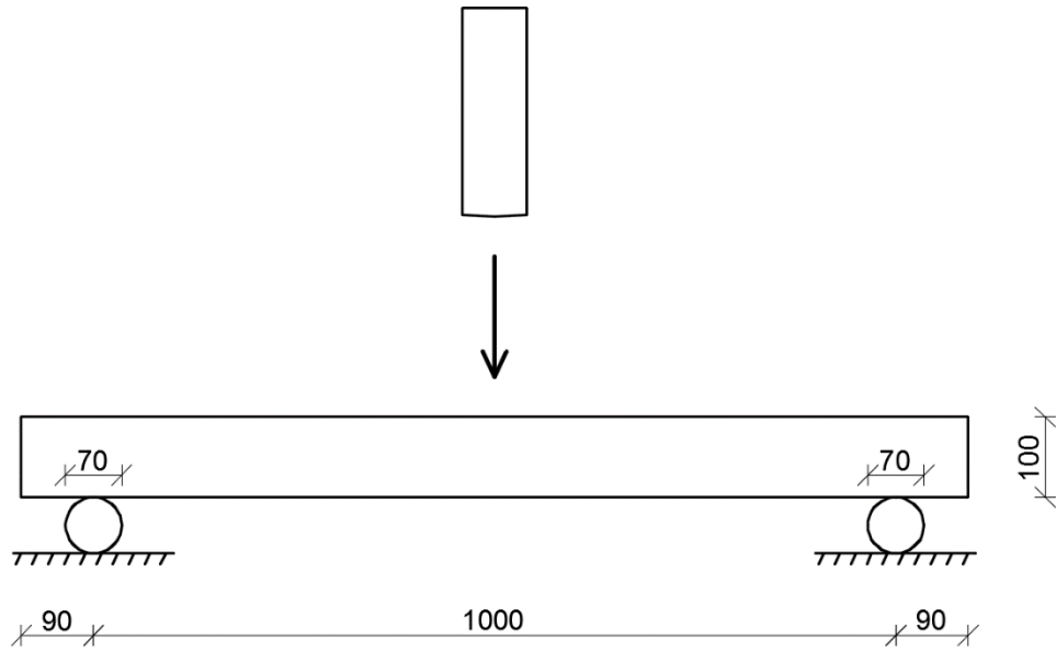
Figure 5.1 Test set up showing the beam geometry and boundary conditions.
