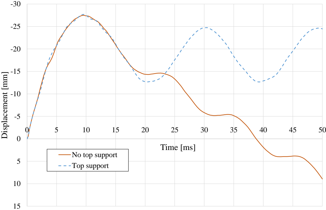
Figure 7.6 Displacement of midpoint as a function of time for two different support conditions.
