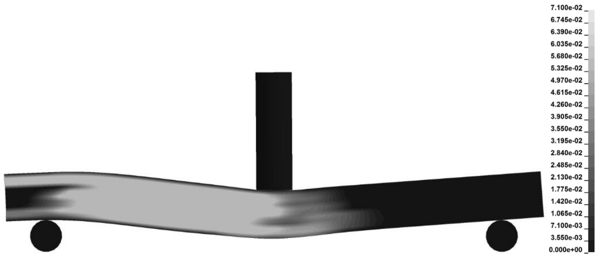
Figure H.8 Beam shape from an LS-DYNA model where the fracture energy input has been reduced by \times 0.5 .
