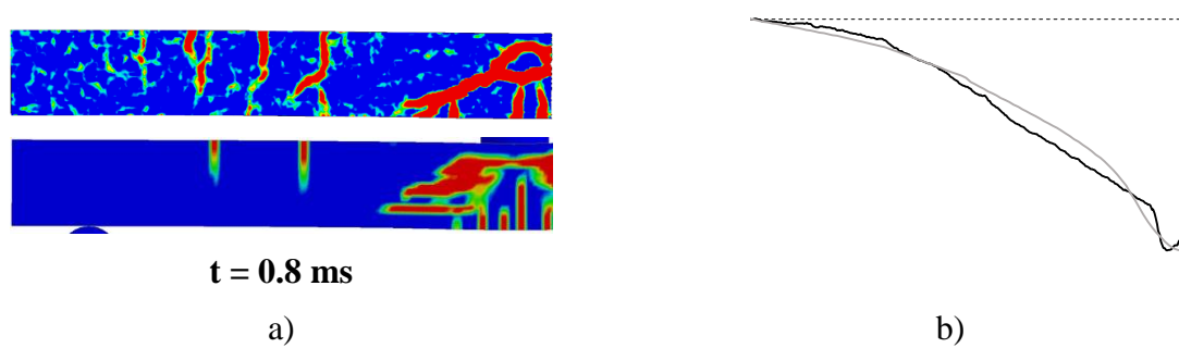
Figure 6.38 Response after 0.8 ms: a) Crack pattern for RPC2 and LS-DYNA, respectively and b) Displacement shape for RPC2 (black) and LS-DYNA (grey).
