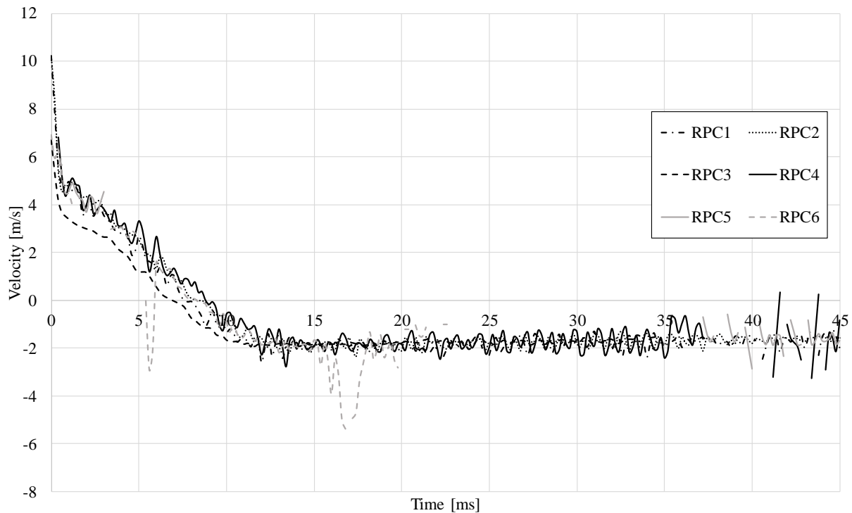
Figure D.24 Drop weight velocity of the beams in the experiment.
