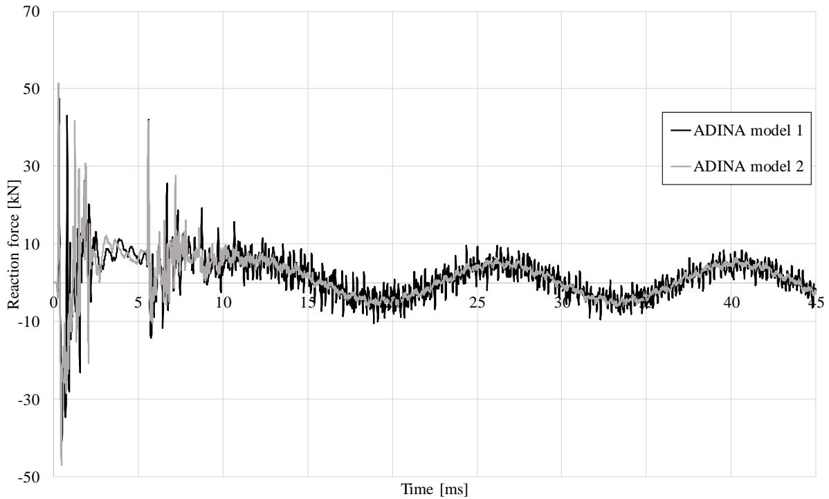
Figure D.10 Reaction force from the supports in the ADINA models.
